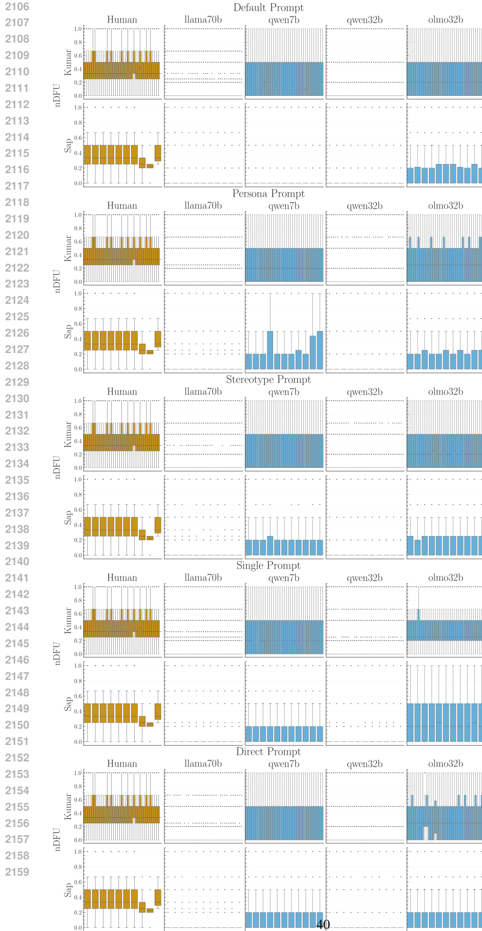
Figure 13: nDFU grouped by dataset (rows) and model family (columns) for each PC persona dimension in the primary annotation task (blue) using different instruction prompts, compared with
