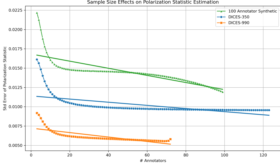
Fig. 10 Standard error of the pol -statistic when sampled with replacement for various number of annotators.
