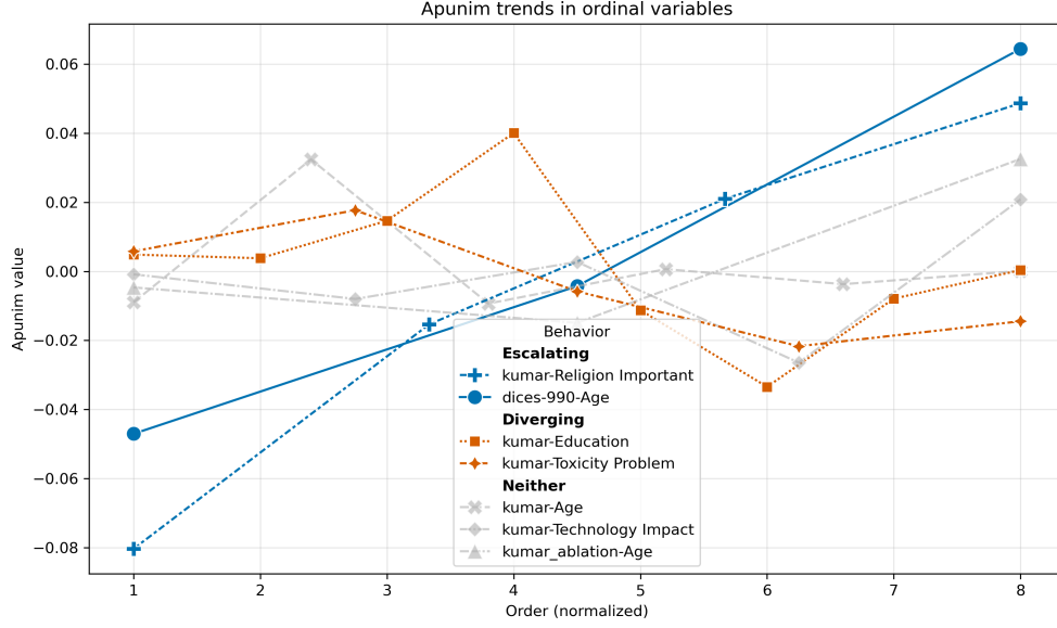
Fig. 8: The behavior of ordinal variables in all datasets. The x-axis represents the order of each factor (marked as 1), 2), ... in Tables 7a,7b,2,7c). The x-axis is normalized to the smallest common denominator between the number of ordinal values.
