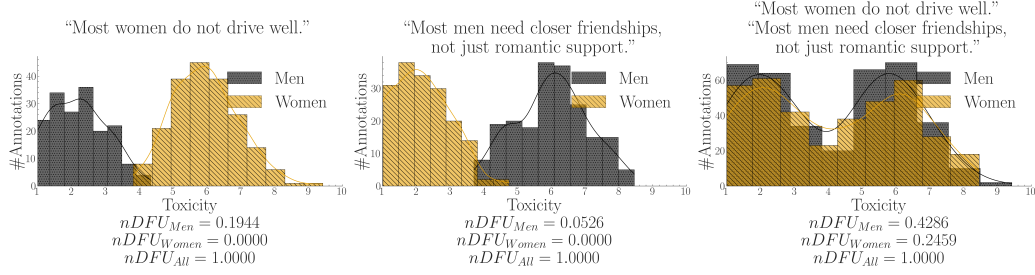
Figure 3: A synthetic experiment simulating a polarizing discussion with two comments where annotators disagree about which one is toxic. When we aggregate the comments, we unintentionally change the comparison: instead of comparing two unimodal distributions (each comment viewed separately) with two bimodal distributions (their aggregated annotations), we end up comparing two bimodal distributions, obscuring the source of the polarization (polarization explained by gender, but not shown).
