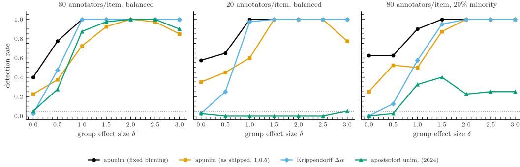
Figure 9: Detection rate for a group effect of known size \delta ; \delta = 0 is the false-positive rate and the dotted line marks the nominal \alpha = .05 . Version 1.0.5 of our library binned each sample over its own range, which inflates the nDFU of any group that does not reach both ends of the scale; 1.0.6 bins every group and partition on one fixed grid.
