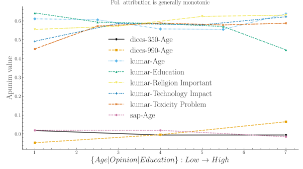
Figure 5: Polarization attribution trends in ordinal groups. The left side of the x-axis (low orders) refers to young annotators, low education, low religiousness, and indifference towards the impacts of toxicity and technology. The full ordinal modes for each dimension and their individual labels can be found in App. F.
