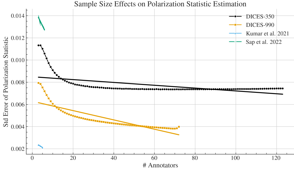
Fig. 8 Std error of the pol-statistic when sampled with replacement for various number of annotators.
