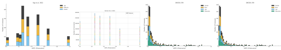
Fig. 6 Histogram of dataset polarization for the human datasets considered in this paper per PC.
