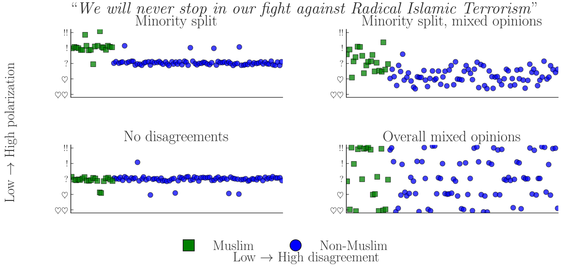
Fig. 1. Simulated experiment exploring four scenarios of a Hate Speech (HS) detection task applied to a controversial statement. The variance in annotations across different annotators may cause traditional Inter-Annotator Agreement (IAA) metrics to ignore minority opinions, especially when opinions are mixed (top-right).
