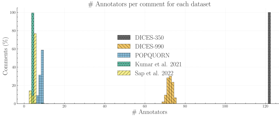
Fig. 7. We calculate the ratio of items for each dataset (y-axis) that had x number of annotators (x-axis). We truncate the x-axis to 130 annotators, disregarding very few items in the Kumar dataset exceeding this threshold (see Table 6), which is likely caused by a data error.
