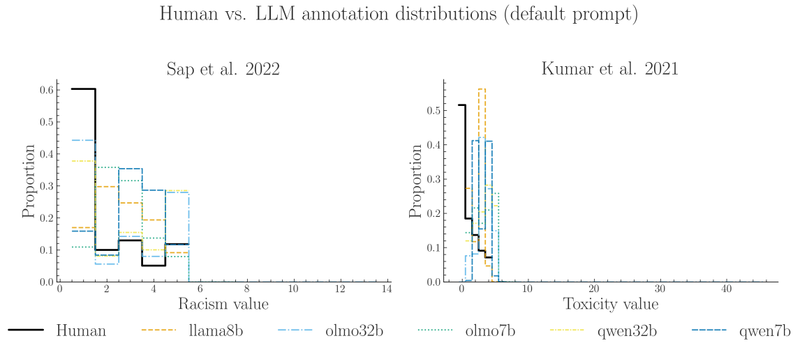
Fig. 10. Annotation frequencies for humans and each LLM in the primary annotation task using the default prompt.
