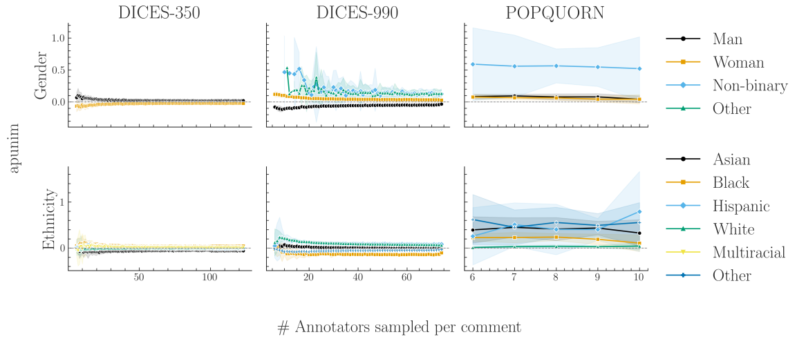
Fig. 5. Standard Deviation (SD) of apunim across items, averaged across 10 runs, where each item is resampled 100 times. Shaded areas represent two SDs. Non-statistically significant results from Table 3 remain systematically close to zero, while statistically significant results can be distinguished from very small annotator counts (six annotators for well-balanced groups, \approx 20 for poorly split groups such as non-binary annotators in DICES-990).
