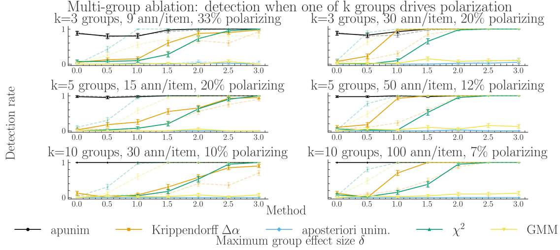
Fig. 8. Polarization group attribution on synthetic distributions. Bars indicate standard error. The setup is identical to the one used for Fig. 2, although in these experiments we consider multiple k annotator groups for each item. Dashed lines show the results of a simplified polarization setup, where polarization always has the same direction.
