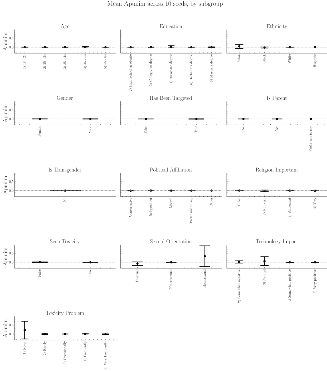
Fig. 9. Apunim values on the Kumar dataset ( n_{samples} = 1000 ) across ten runs with different subsets. Black bars indicate two SDs. PC dimensions with many groups are more volatile, although all dimensions broadly keep the same apunim sign across subsets.
