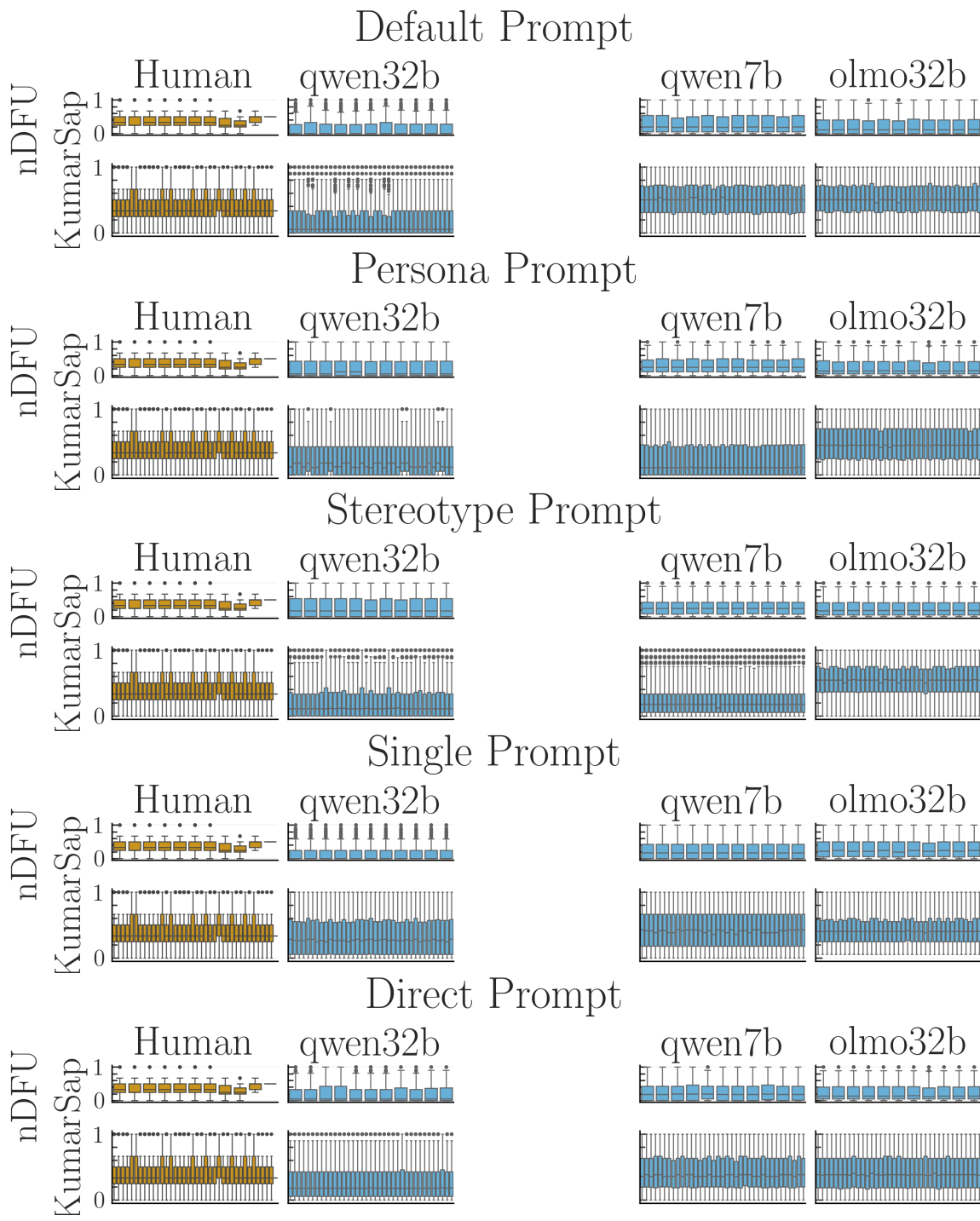
Fig. 11. nDFU grouped by dataset (rows) and model family (columns) for each PC persona dimension in the primary annotation task (blue) using different instruction prompts, compared with human annotations on the same sample (yellow).
