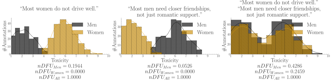
Fig. 3. Synthetic experiment showing two comments with annotators disagreeing about which one is toxic. Instead of comparing two unimodal distributions (comments viewed separately) with two bimodal distributions (their aggregated annotations), we end up comparing two bimodal distributions during aggregation, obscuring the source of the polarization (explained by gender, but not shown).
