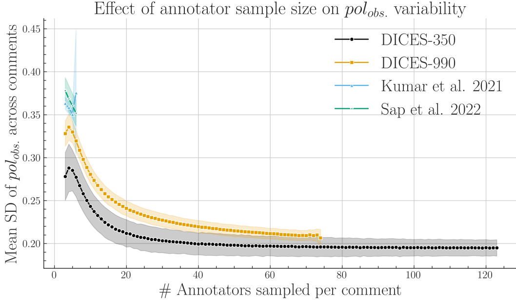
Figure 11: SD of pol_{obs} across items, averaged across 1000 runs (Eq. 6). Shaded areas represent two SDs. Pol. estimates benefit from more annotators up to n = 20 , at which point they begin to plateau.
