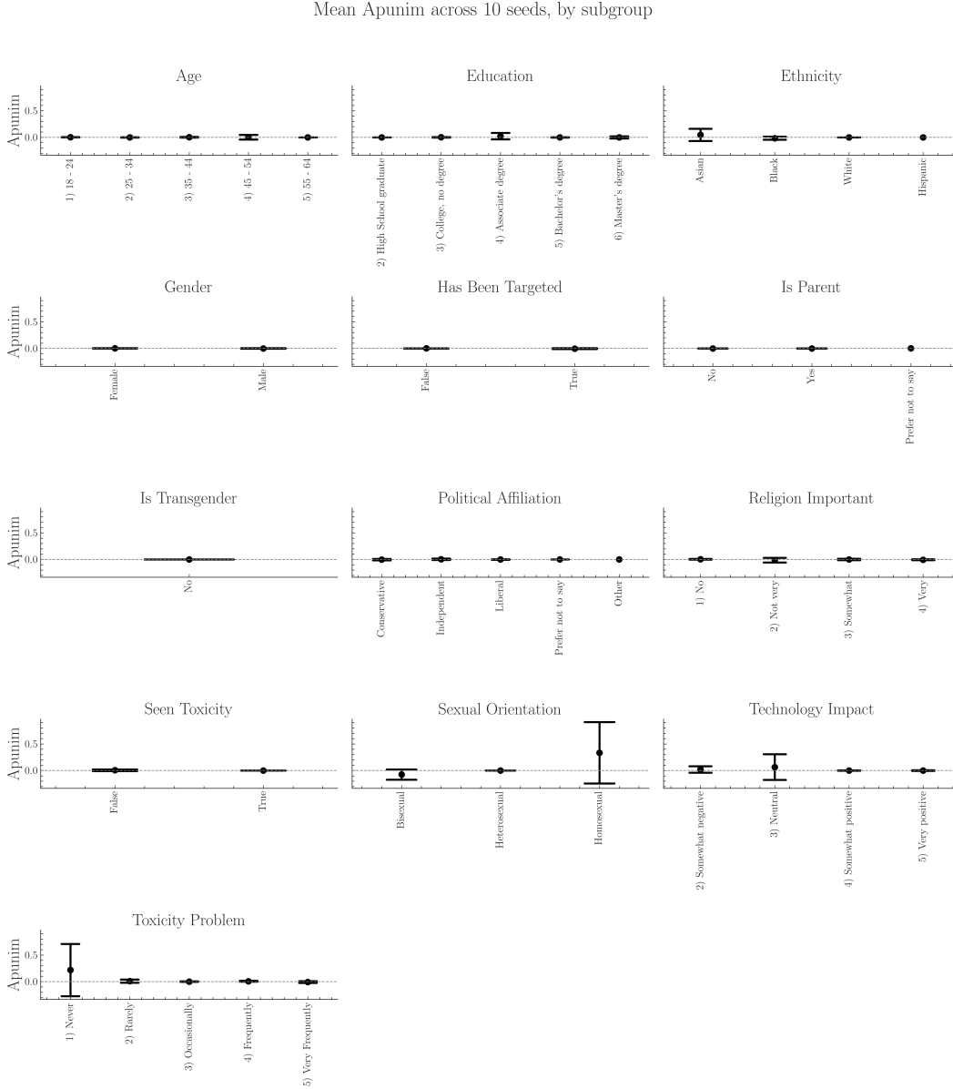
Figure 8: Apunim values on the Kumar dataset ( n_{samples} = 1000 ) across ten runs with different subsets. Black bars indicate two SDs. PC dimensions with many groups are more volatile, although all dimensions broadly keep the same apunim sign across subsets.
