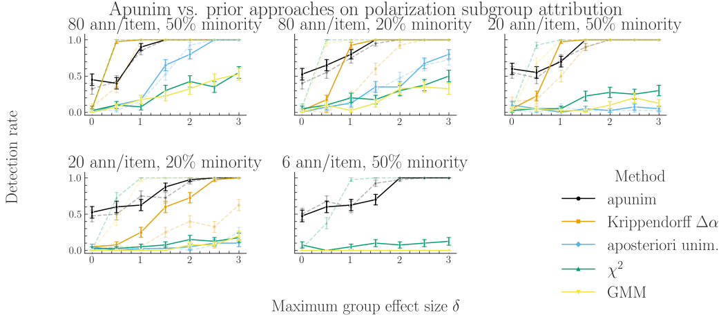
Figure 2: Polarization group attribution on synthetic distributions. Bars indicate standard error. We assign a number of annotators per item, and split the annotator groups 50-50 or 80-20. Higher \delta represents higher polarization. Apunim is adept at attributing polarization to the correct group regardless of number of annotators per item, or how these annotators are split. Dashed lines show the results of a simplified polarization setup, where polarization always has the same direction.
