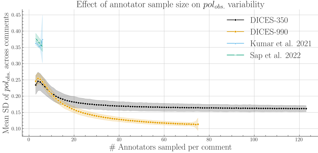
Figure 11: SD of pol_{obs} across items, averaged across 1000 runs. Shaded areas represent two SDs. Pol. estimates benefit from more annotators up to n = 20 , at which point they begin to plateau.
