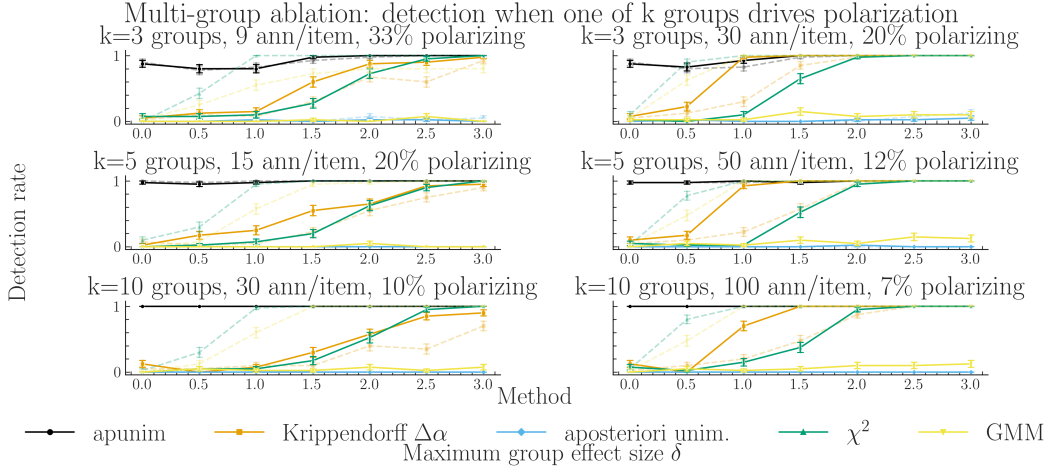
Figure 7: Polarization group attribution on synthetic distributions. Bars indicate standard error. The setup is identical to the one used for Fig. 2, although in these experiments we consider multiple k annotator groups for each item. Dashed lines show the results of a simplified polarization setup, where polarization always has the same direction.
