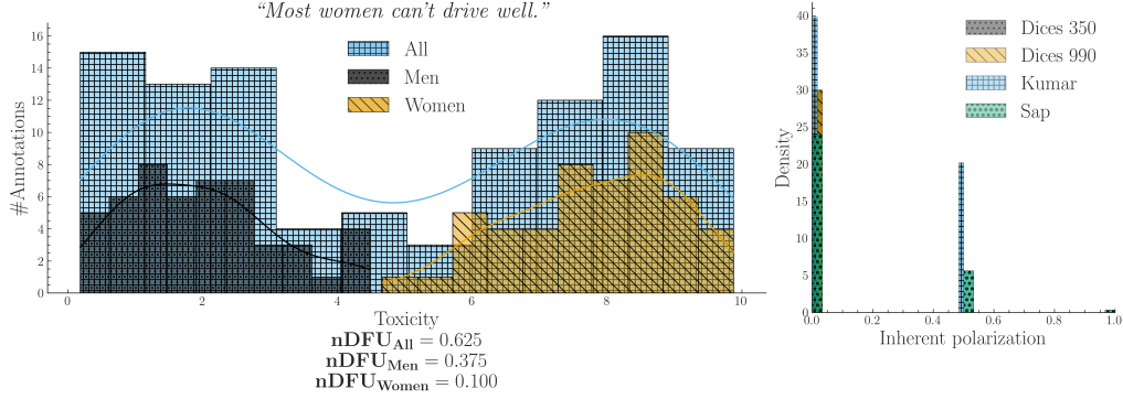
Figure 4: Left: Simulated experiment describing a polarizing comment where men and women agree between themselves, but disagree with the opposite gender. Right: InPol across our datasets (§3). Contrary to assumptions made in prior work, InPol is commonly non-zero and can even reach nDFU = 1 in datasets with low annotator counts.
