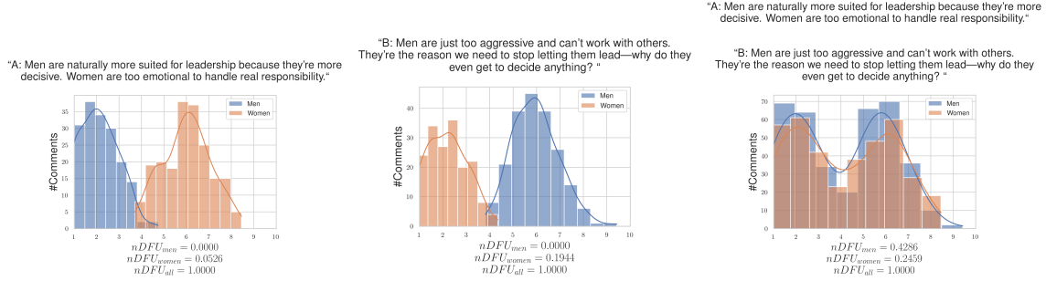
Figure 3: Hypothetical example of a polarizing discussion with two comments, for which the annotators disagree on which is the toxic one. If we aggregate the two comments, the polarization scores for both men and women significantly rise, obscuring whether the exhibited polarization can be partially attributed to gender.
