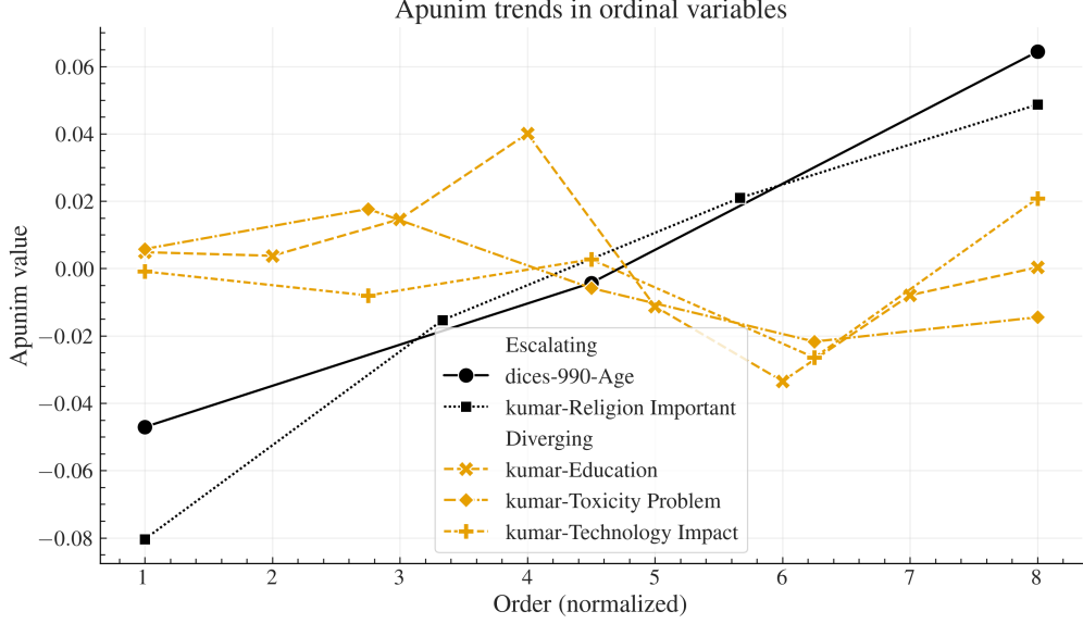
Fig. 6 Apunim values across ordinal factor levels with at least two statistically significant values. The x-axis corresponds to the ordered levels of each factor and is normalized so that different ordinal scales are comparable (e.g., education which is measured in different scales across datasets). The left side of the x-axis (low orders) refers to young annotators, low education, low religiousness, and indifference towards the impacts of toxicity and technology. The full ordinal modes for each dimension can be found in Appendix E.
