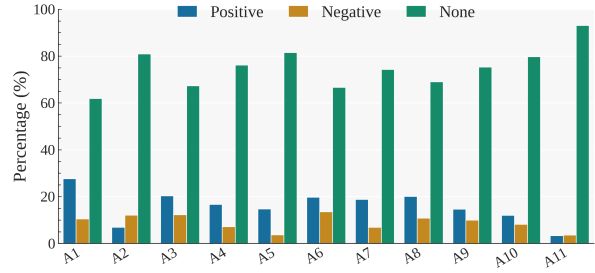
Figure 5: Distribution of all classes per annotator.
