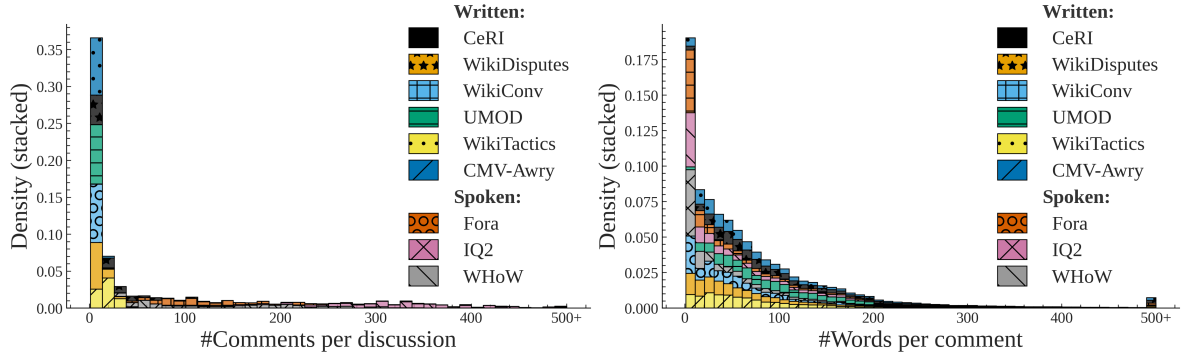
Figure 2: Left: Comments per discussion on the PEFK dataset. Note the significant increase in comments made in transcribed datasets such as Fora and IQ2. This deviation is explained by the fact that a single human utterance is regularly broken up to many comments in order to simulate interruptions or participants talking over each other. Right: Number of words per comment in all discussions in PEFK , grouped by original dataset. Comments across written datasets follow the same distribution, while spoken datasets feature a significant number of comments with very few words.
