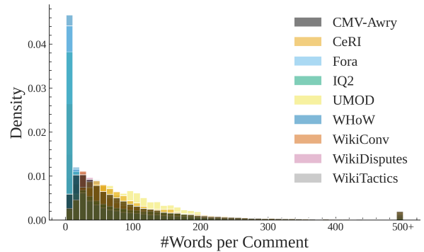
Figure 7: Number of words per comment in all discussions on the PEFK dataset, grouped by original dataset. Comments across written datasets follow the same distribution, while spoken datasets feature a significant number of comments with very few words.
