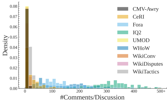
Figure 6: Comments per discussion on the PEFK dataset. Note the significant increase in comments made in transcribed datasets such as Fora and IQ2. This deviation is explained by the fact that a single human utterance is regularly broken up to many comments in order to simulate interruptions or participants talking over each other.
