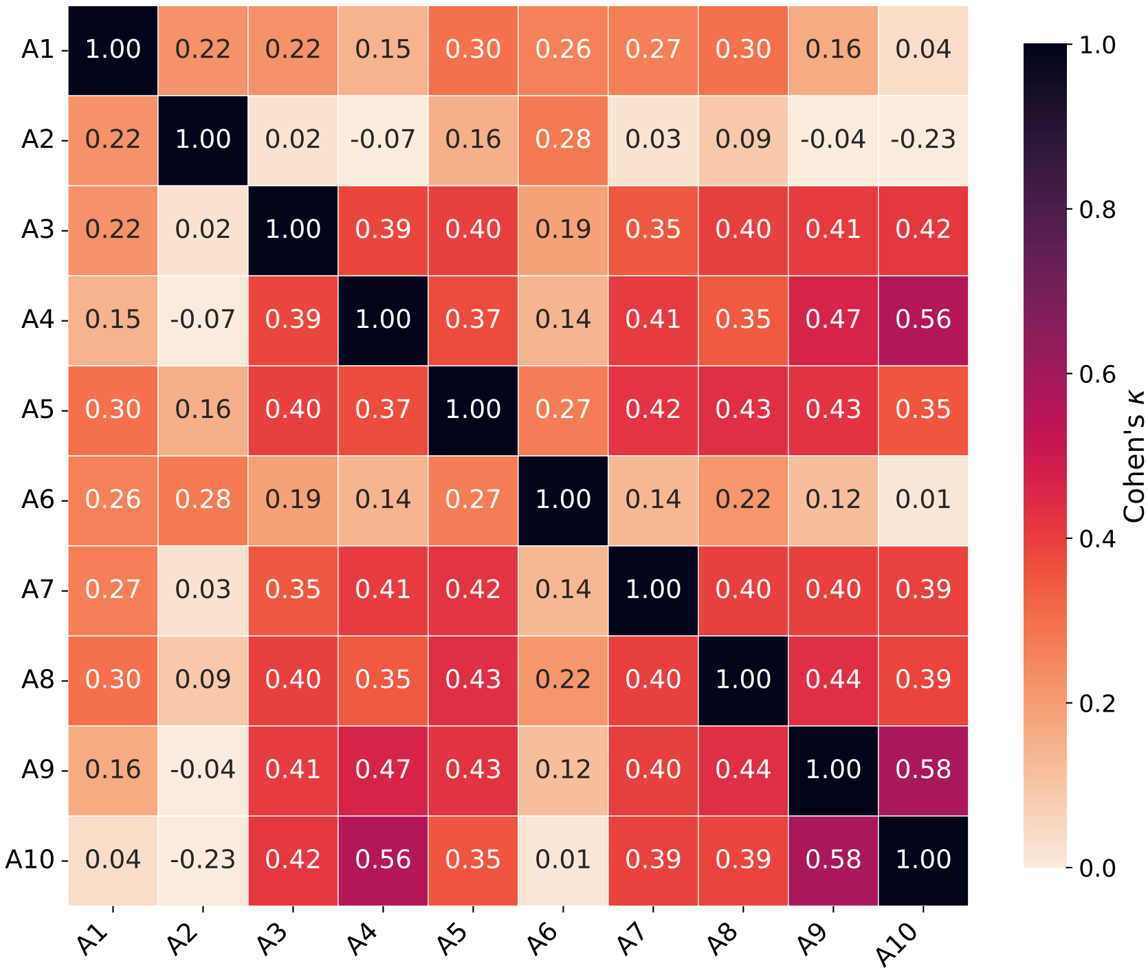
Pairwise Cohen's Kappa Between Annotators (binary \geq 3 )
