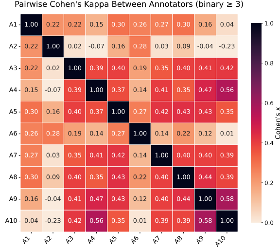
Figure 3: Heatmap of pairwise Cohen’s \kappa scores.
