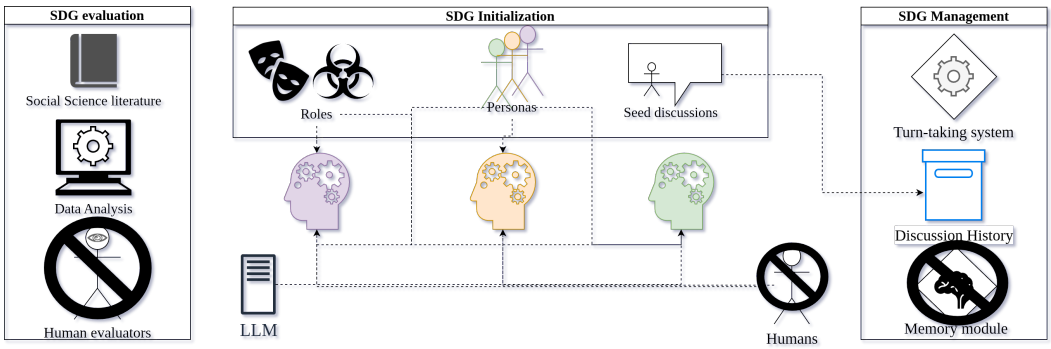
Fig. 2. We design SDG systems through three high-level components: (1) the creation of LLM participants in lieu of humans (§3.2), (2) simple synthetic systems that handle conversational dynamics (§3.3), and (3) scalable evaluation methodologies grounded in literature which avoid human validation as much as possible (§3.4).
