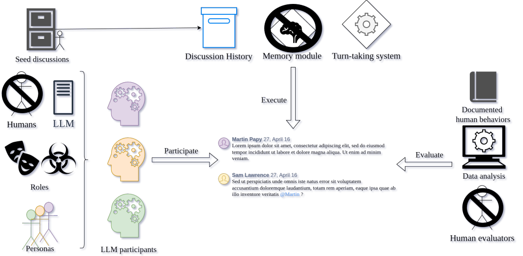
Fig. 2. We design SDG systems through three high-level components: (1) the creation of LLM participants in lieu of humans (§3.2), (2) simple synthetic systems that handle conversational dynamics (§3.3), and (3) scalable evaluation methodologies grounded in literature which avoid human validation as much as possible (§3.4).
