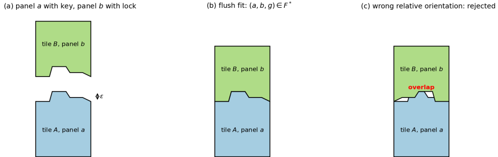
Figure 3: Keys and locks in cross-section. (a) An asymmetric relief of height \varepsilon on panel a (key) and its complement on panel b (lock). (b) The two panels fit flush only in the relative orientations g for which (a, b, g) \in F^* . (c) In any other relative orientation the reliefs overlap, so the placement is impossible.
