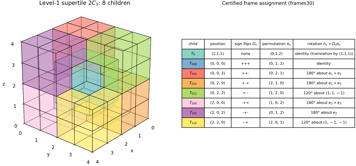
Figure 1: Left: the level-1 supertile 2C_3 and its eight children, viewed from the socket side. Tiles are drawn semi-transparent with only their outlines, so the shape of every chair can be seen: the central translate T_0 (teal) sits at the bottom of the socket and the child T_{000} (blue) is at the back, visible through the front tiles. Right: the certified frame assignment. “Position” is the corner 2v of the 2 \times 2 \times 2 block B_v = 2v + [0, 2]^3 occupied by the child, i.e. the (x, y, z) coordinates of the lowest corner of its bounding cube in units of unit cubes (for T_0 it is the translation vector (1, 1, 1)). Permutations are written as tuples \pi = (\pi(0), \pi(1), \pi(2)) acting on 0-indexed coordinates; the sign flips are D_{s(v)} . All eight child maps are proper rotations (homochiral).
