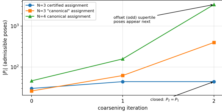
Figure 2: Coarsening iteration |P_i| for three assignments. The certified 3D assignment closes ( 30 \rightarrow 44 \rightarrow 44 ). The “canonical” assignments (sign flips composed with a fixed transposition where a rotation is required) do not: the closure grows and then admits offset supertile poses, in N = 3 and N = 4 alike.
