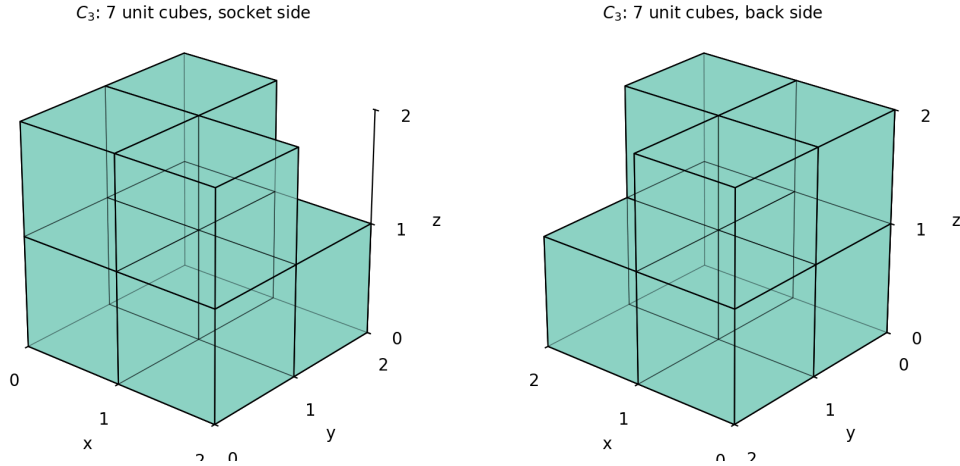
Figure 1: The three-dimensional chair C_3 , the shape of the Chair44 tile: the cube [0, 2]^3 with the unit corner cube (1, 2]^3 removed, seen from the socket side (left) and from the back (right). Faint lines mark the seven unit cubes.
