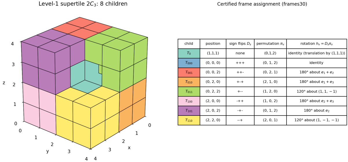
Figure 2: Left: the level-1 supertile 2C_3 and its eight children, viewed from the socket side. The central translate T_0 (teal) is visible at the bottom of the socket; the child T_{000} (blue) is at the back and hidden. Right: the certified frame assignment. “Position” is the corner 2v of the 2 \times 2 \times 2 block B_v = 2v + [0, 2]^3 occupied by the child, i.e. the (x, y, z) coordinates of the lowest corner of its bounding cube in units of unit cubes (for T_0 it is the translation vector (1,1,1)). Permutations are written as tuples \pi = (\pi(0), \pi(1), \pi(2)) acting on 0-indexed coordinates; the sign flips are D_{s(v)} . All eight child maps are proper rotations (homochiral).
