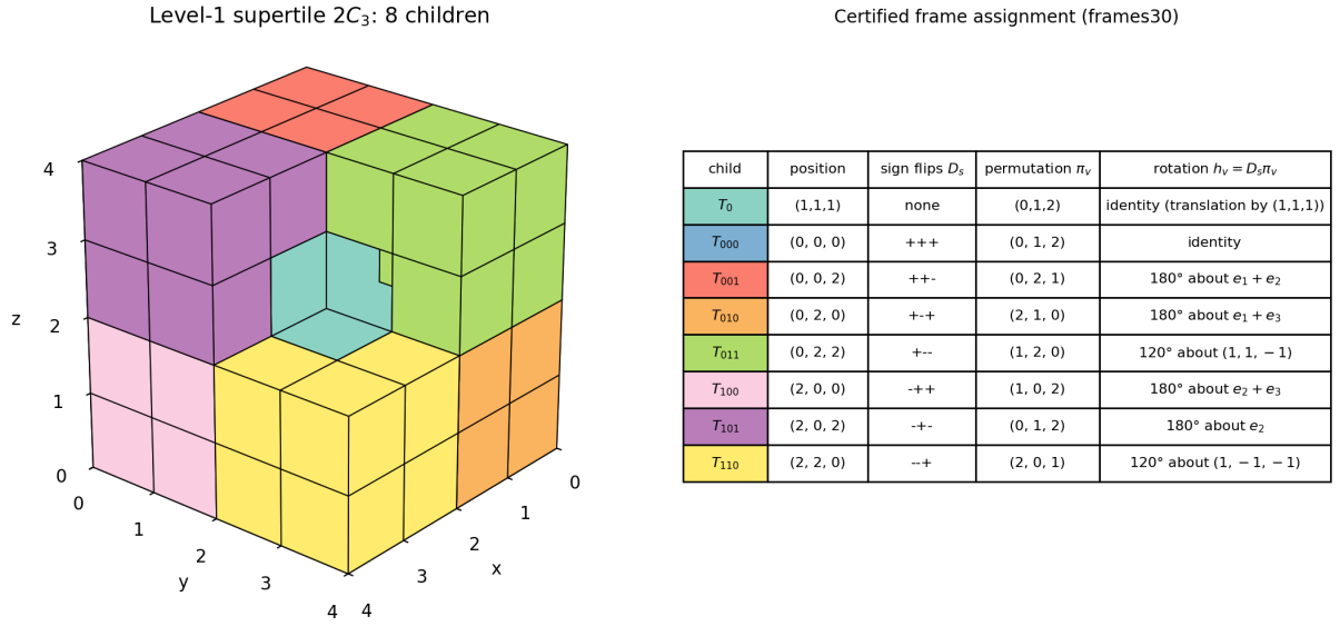
Figure 3: Left: the level-1 supertile 2C_3 and its eight children, viewed from the socket side. The central translate T_0 (teal) is visible at the bottom of the socket; the child T_{000} (blue) is at the back and hidden. Right: the certified frame assignment. “Position” is the corner 2v of the 2 \times 2 \times 2 block B_v = 2v + [0, 2]^3 occupied by the child, i.e. the (x, y, z) coordinates of the lowest corner of its bounding cube in units of unit cubes (for T_0 it is the translation vector (1,1,1)). Permutations are written as tuples \pi = (\pi(0), \pi(1), \pi(2)) acting on 0-indexed coordinates; the sign flips are D_{s(v)} . All eight child maps are proper rotations (homochiral).
