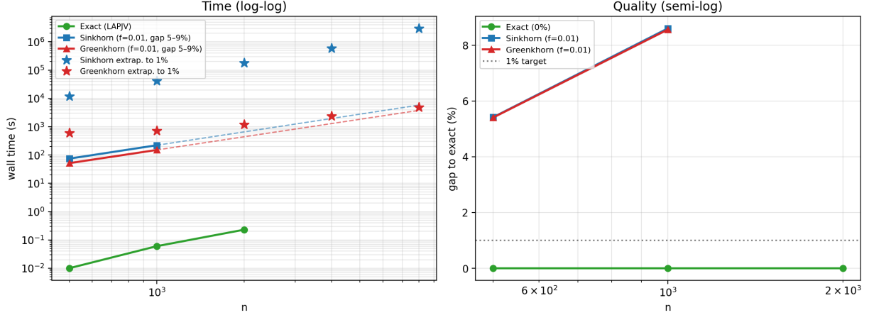
Figure 1: Exact (Jonker–Volgenant) vs vanilla Sinkhorn and Greenkhorn on the dense uniform grid (seed 7). Solid lines are measured wall times at f = 0.01 where each approximate method produces a transport plan 5–9% above the exact optimum. Dashed lines continue the empirical log-log slope of those measured curves; star markers are the rough Table 3 extrapolation to the 1% quality target. Exact is below both approximate curves at every measured n in both time and quality.
