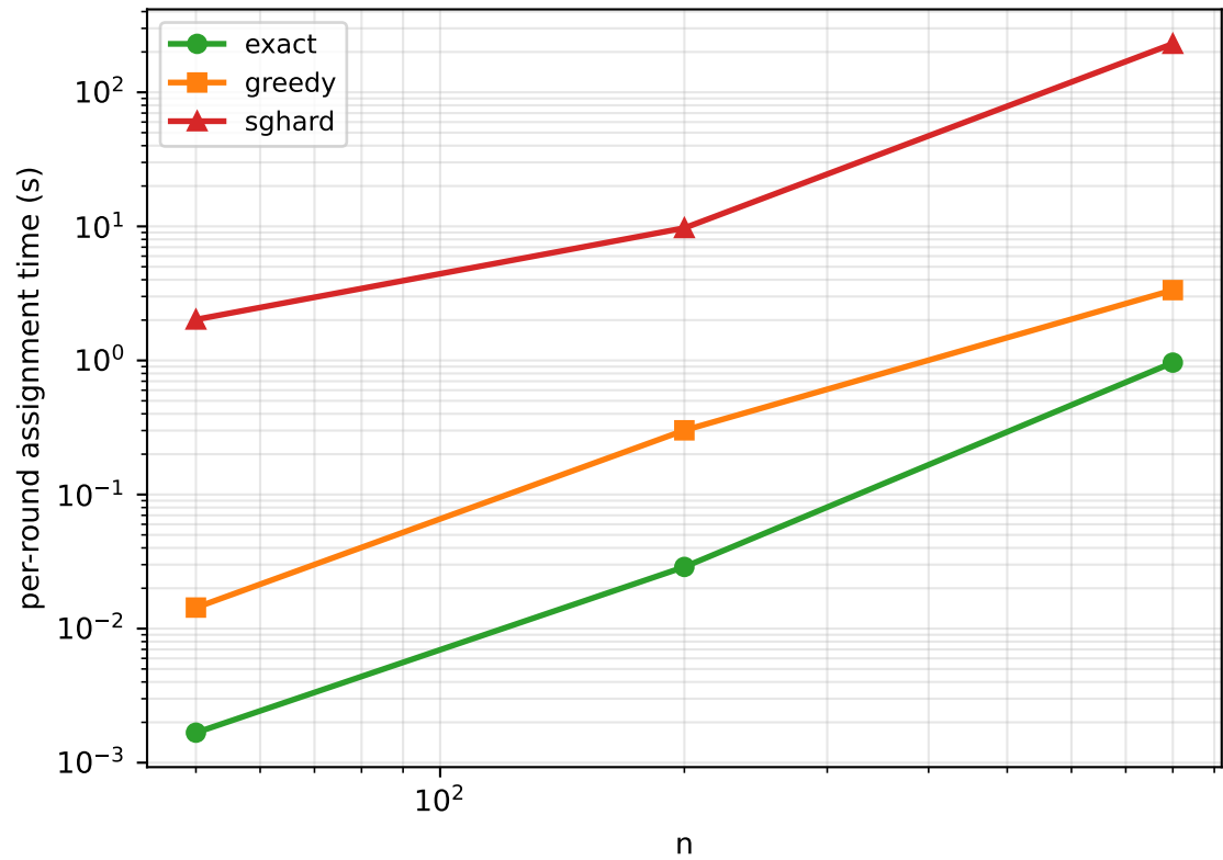
Per-round assignment cost (log scale)
