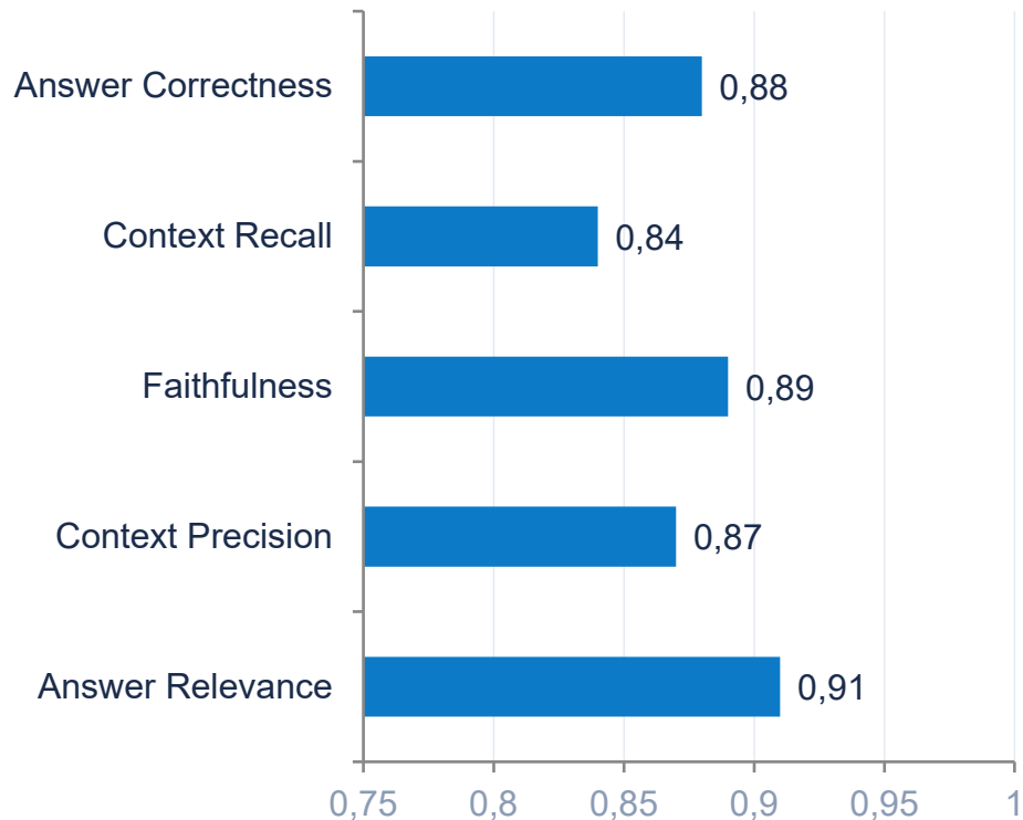
RAG Evaluation Scores
