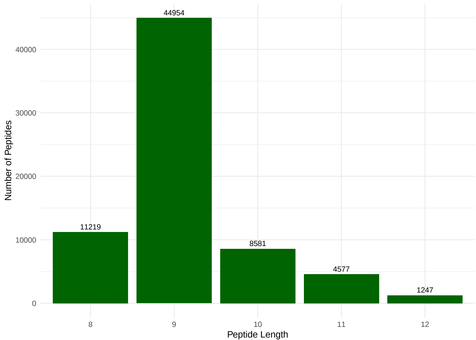
Peptide Length Distribution
