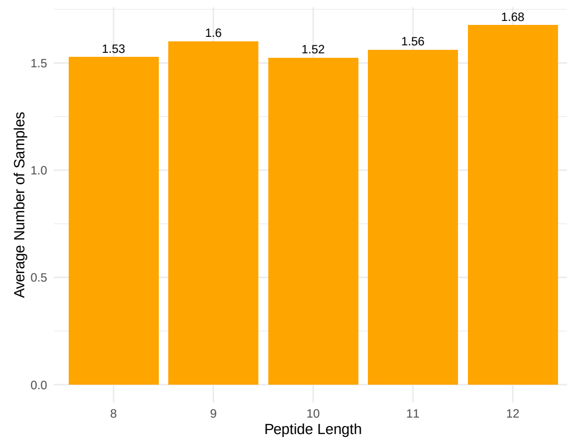
Average Sharing by Peptide Length
