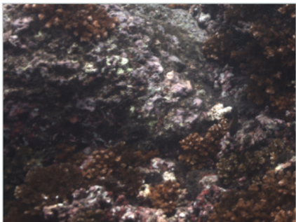
Panama
