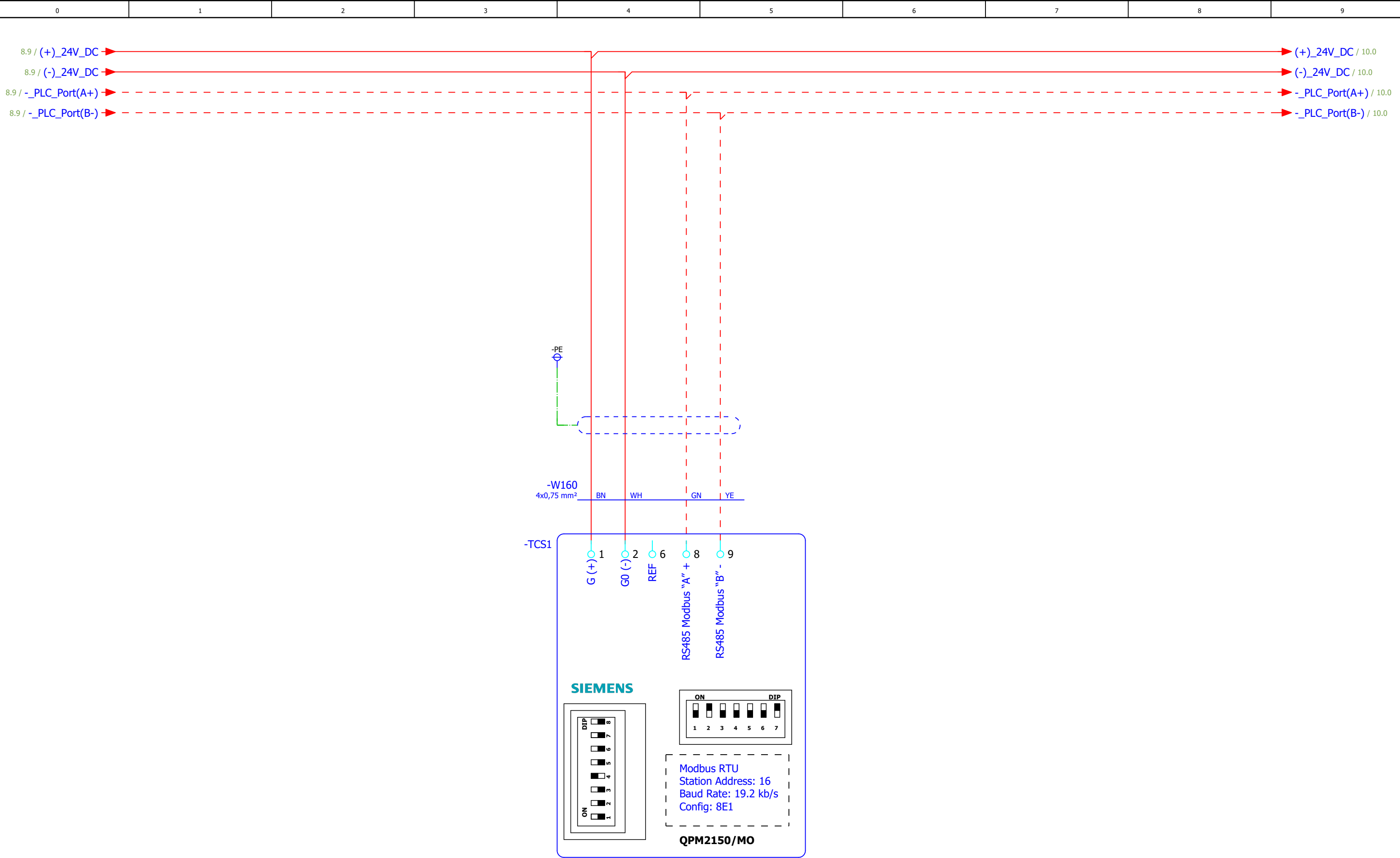
Return Air CO 2 And Temperature Sensor
