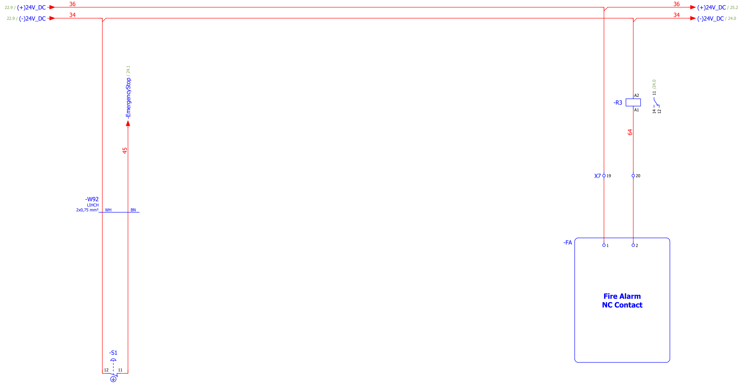
Fire Alarm Relay
