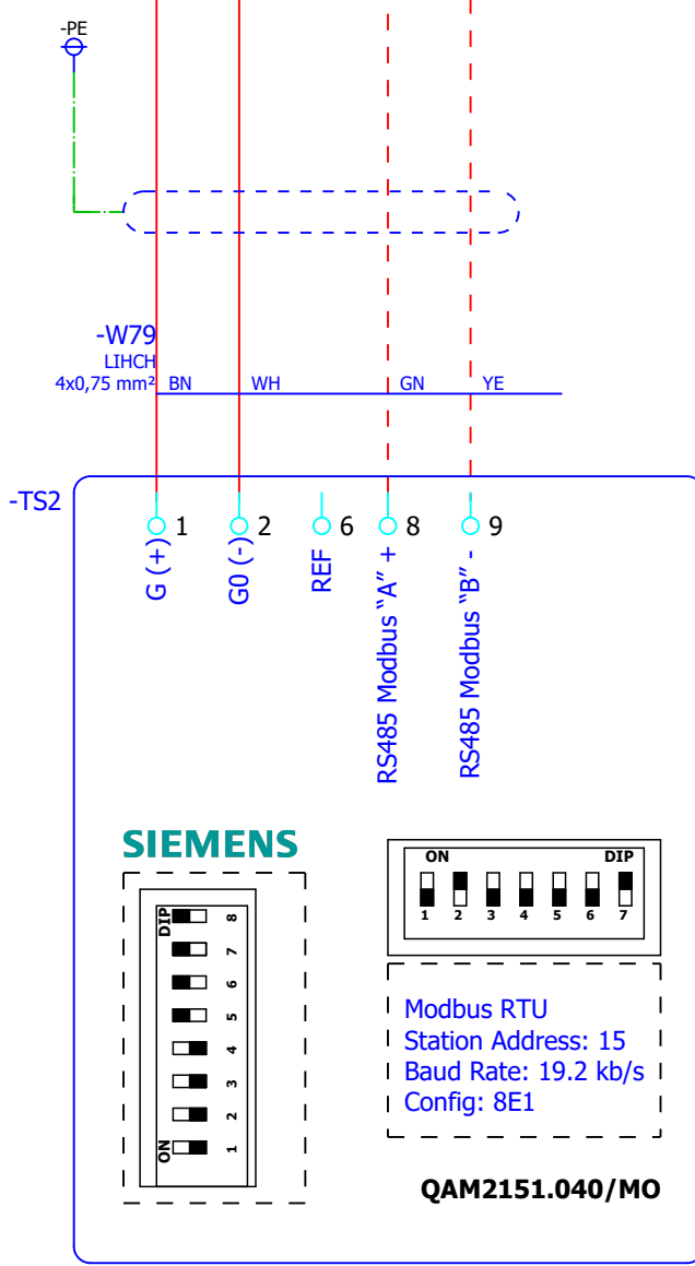
After DX Unit Temperature Sensor
