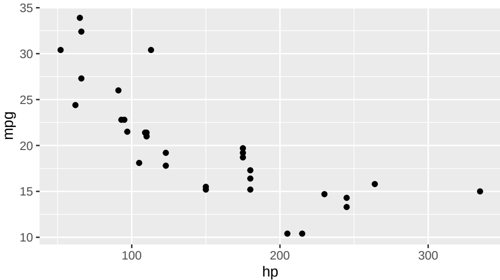
Miles per Gallon vs Horsepower
