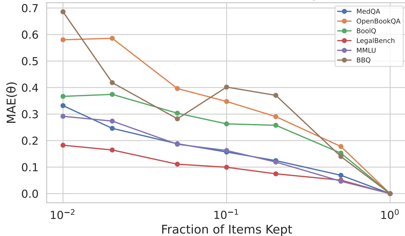
\theta Estimation Error vs. Item Budget
