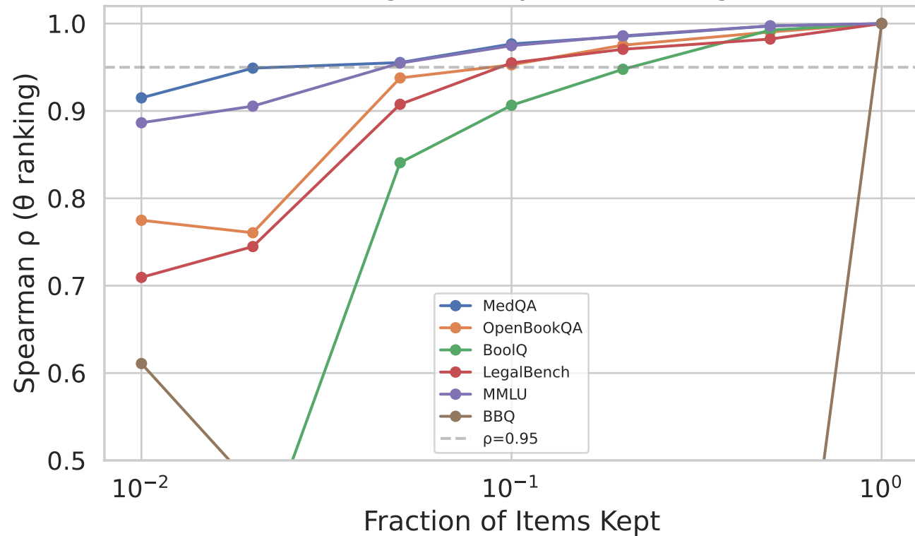
\theta Ranking Recovery vs. Item Budget
