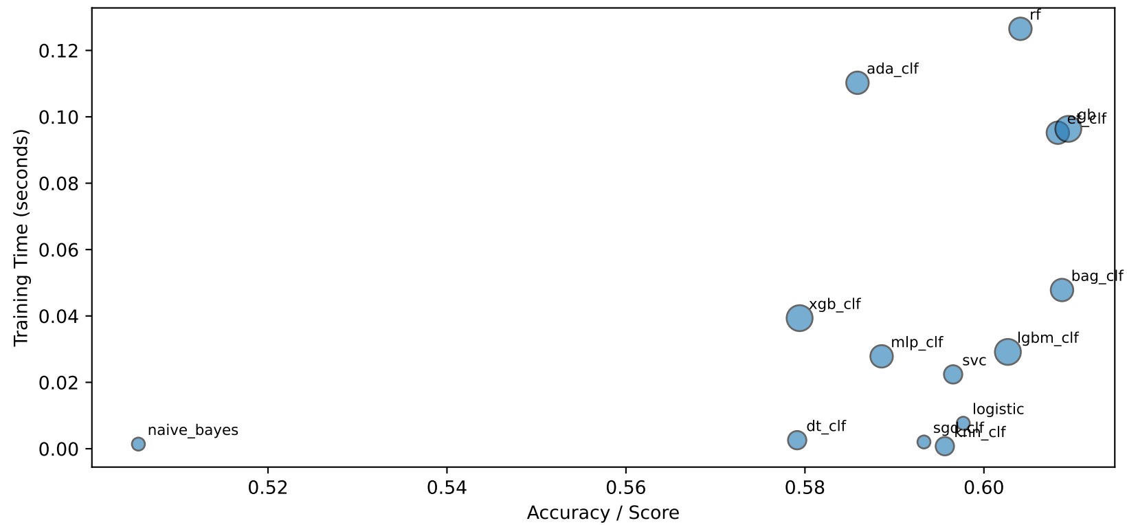
Dataset 1480 (Classification) - Model Trade-offs
