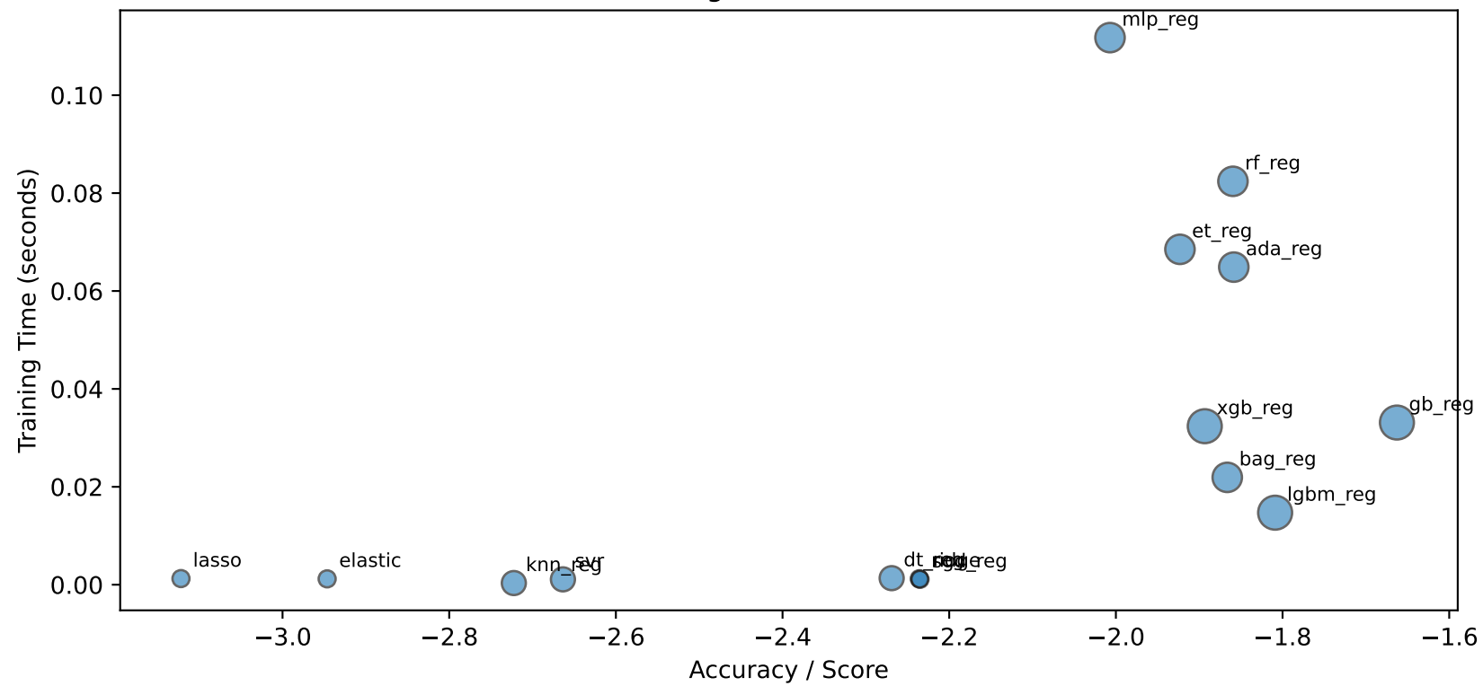
Dataset 229 (Regression) - Model Trade-offs
