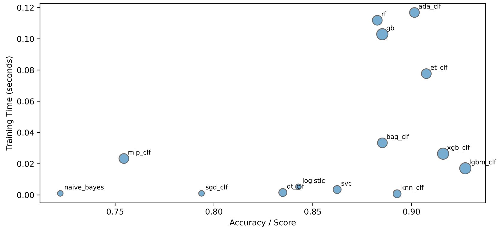
Dataset 1488 (Classification) - Model Trade-offs
