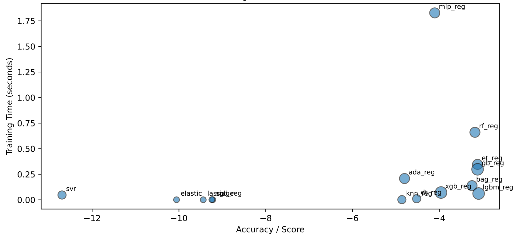
Dataset 227 (Regression) - Model Trade-offs
