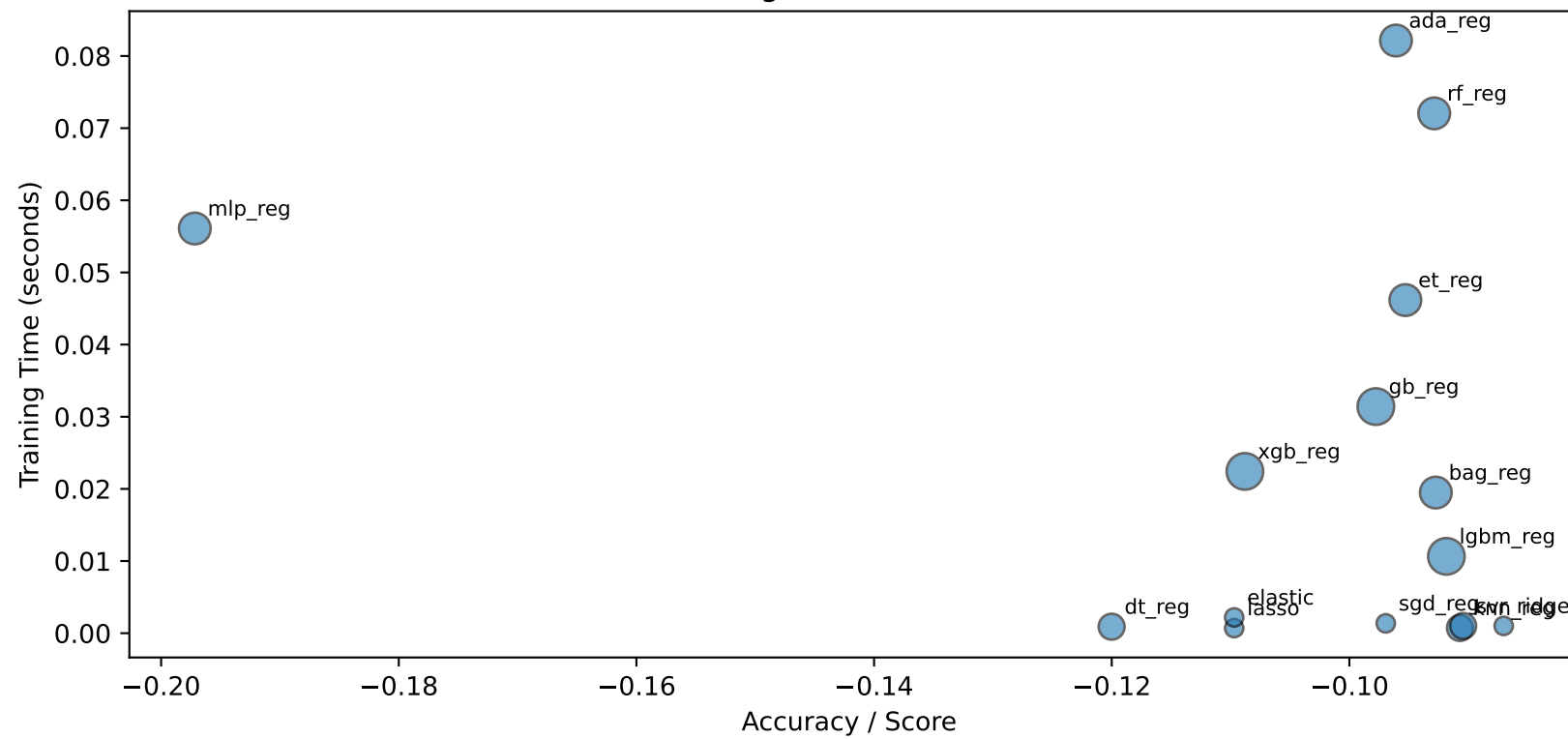
Dataset 214 (Regression) - Model Trade-offs
