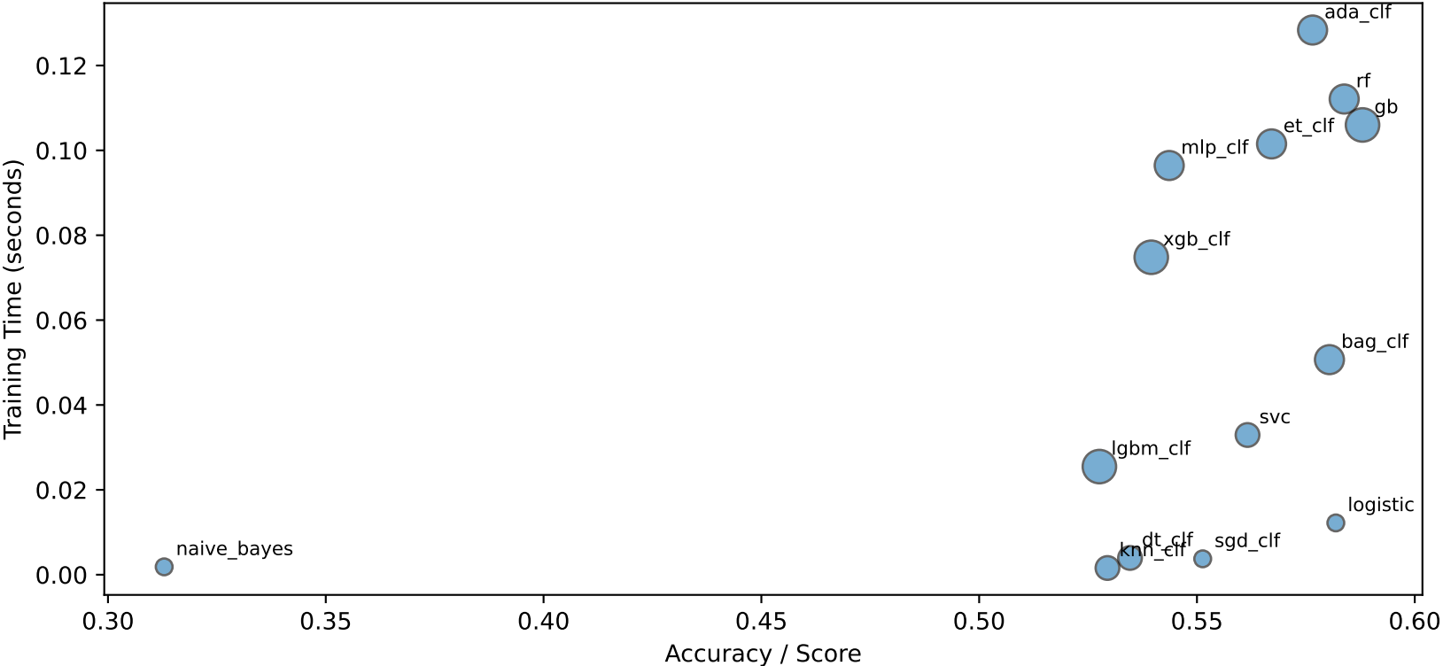
Dataset 23381 (Classification) - Model Trade-offs
