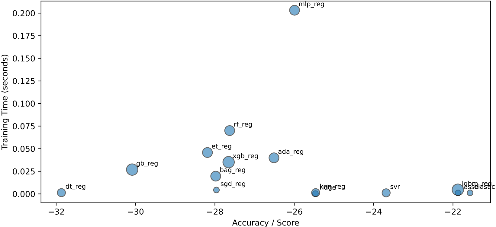
Dataset 228 (Regression) - Model Trade-offs
