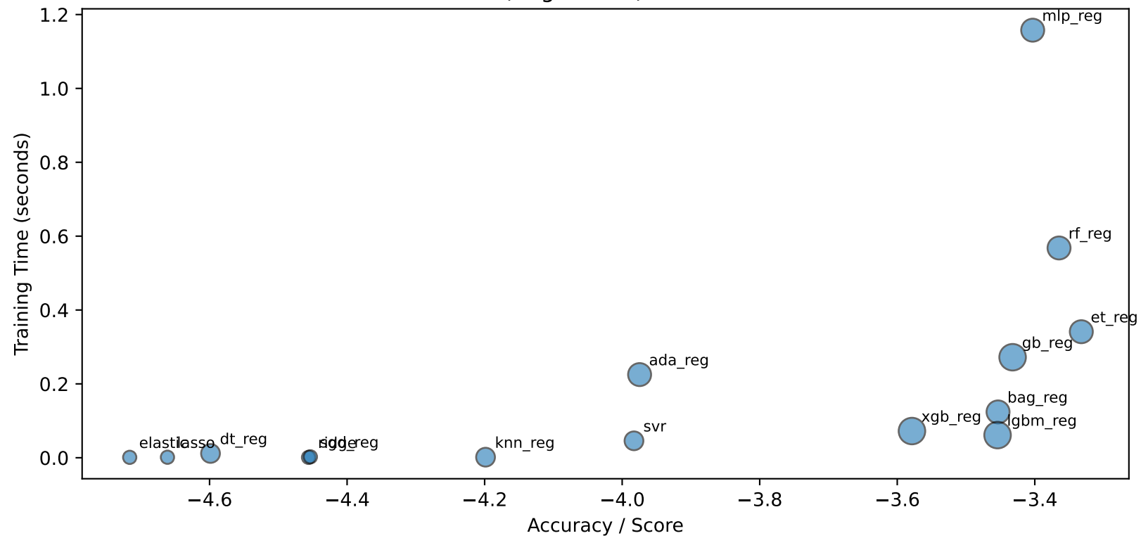
Dataset 225 (Regression) - Model Trade-offs
