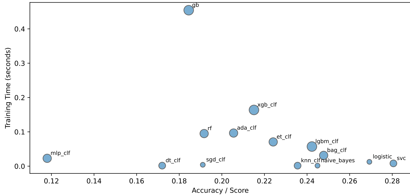
Dataset 1027 (Classification) - Model Trade-offs
