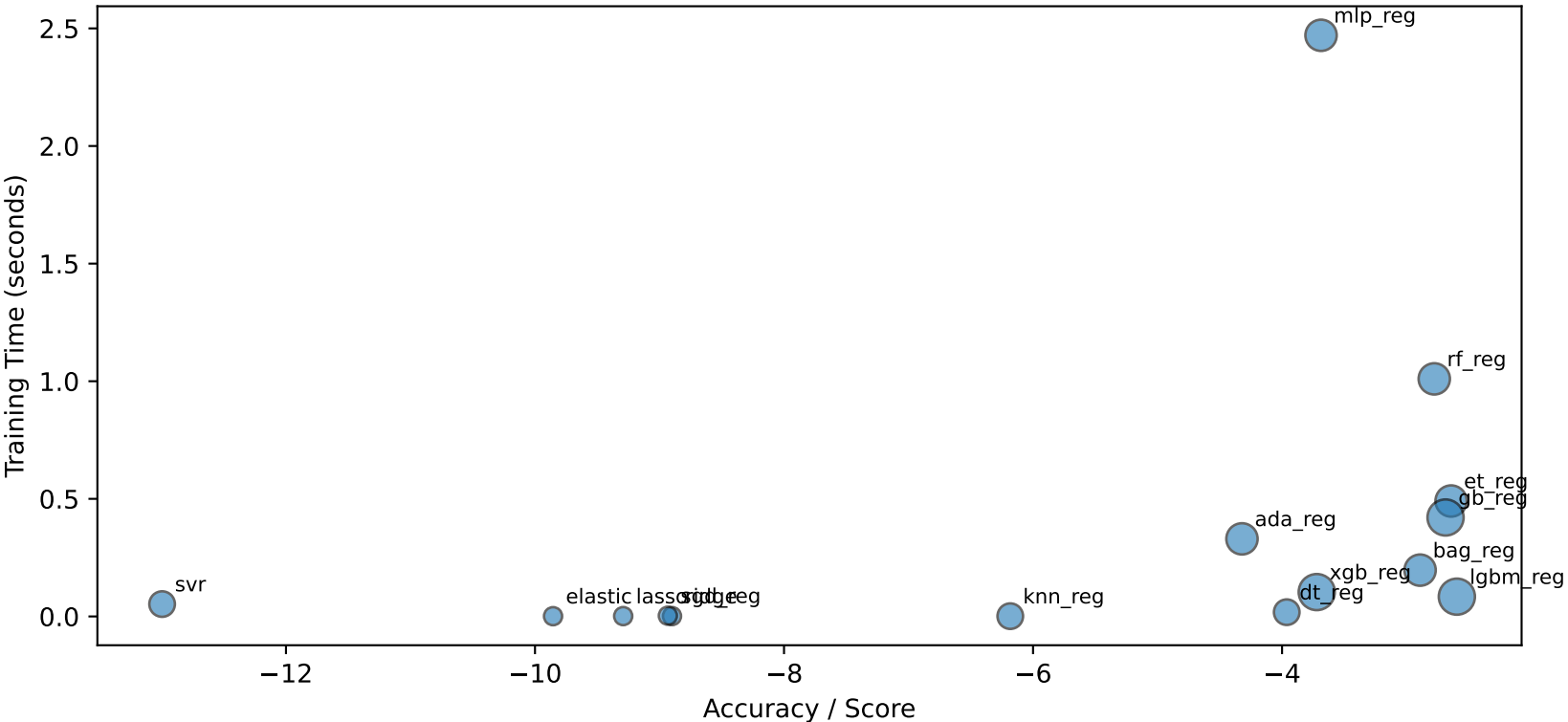
Dataset 197 (Regression) - Model Trade-offs
