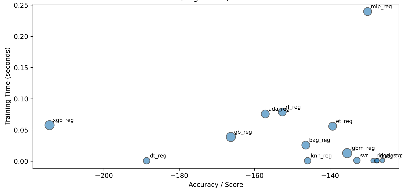
Dataset 230 (Regression) - Model Trade-offs
