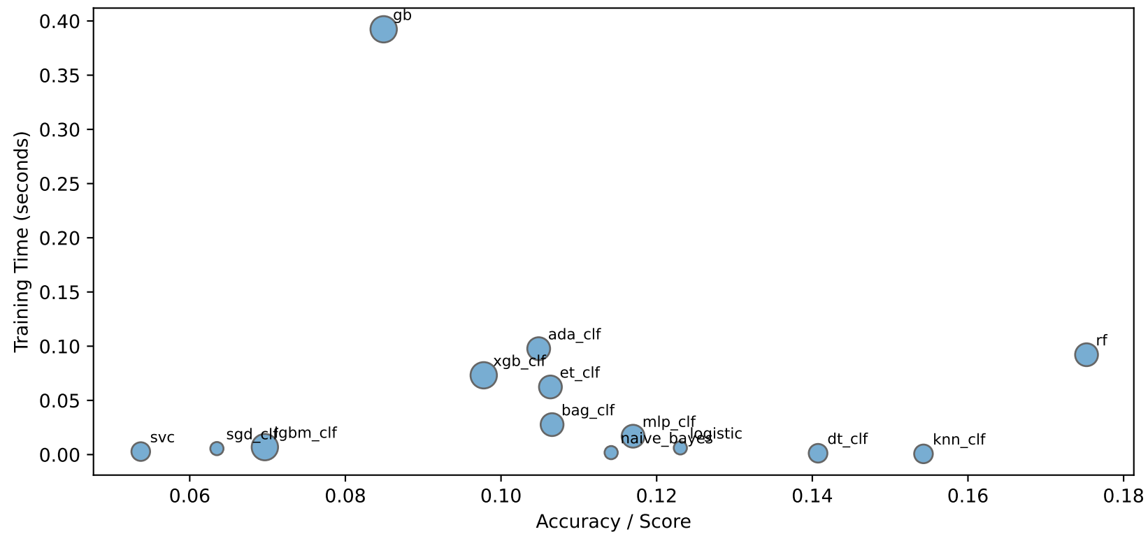
Dataset 1030 (Classification) - Model Trade-offs
