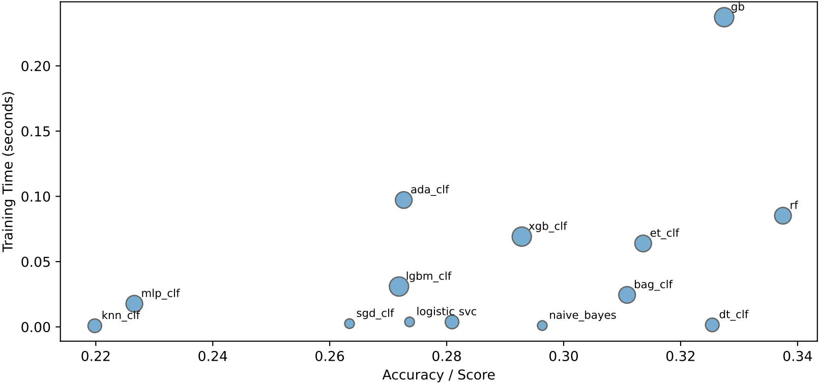
Dataset 1029 (Classification) - Model Trade-offs
