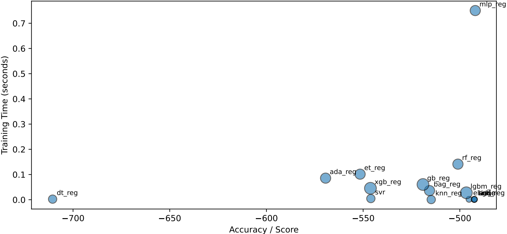
Dataset 549 (Regression) - Model Trade-offs
