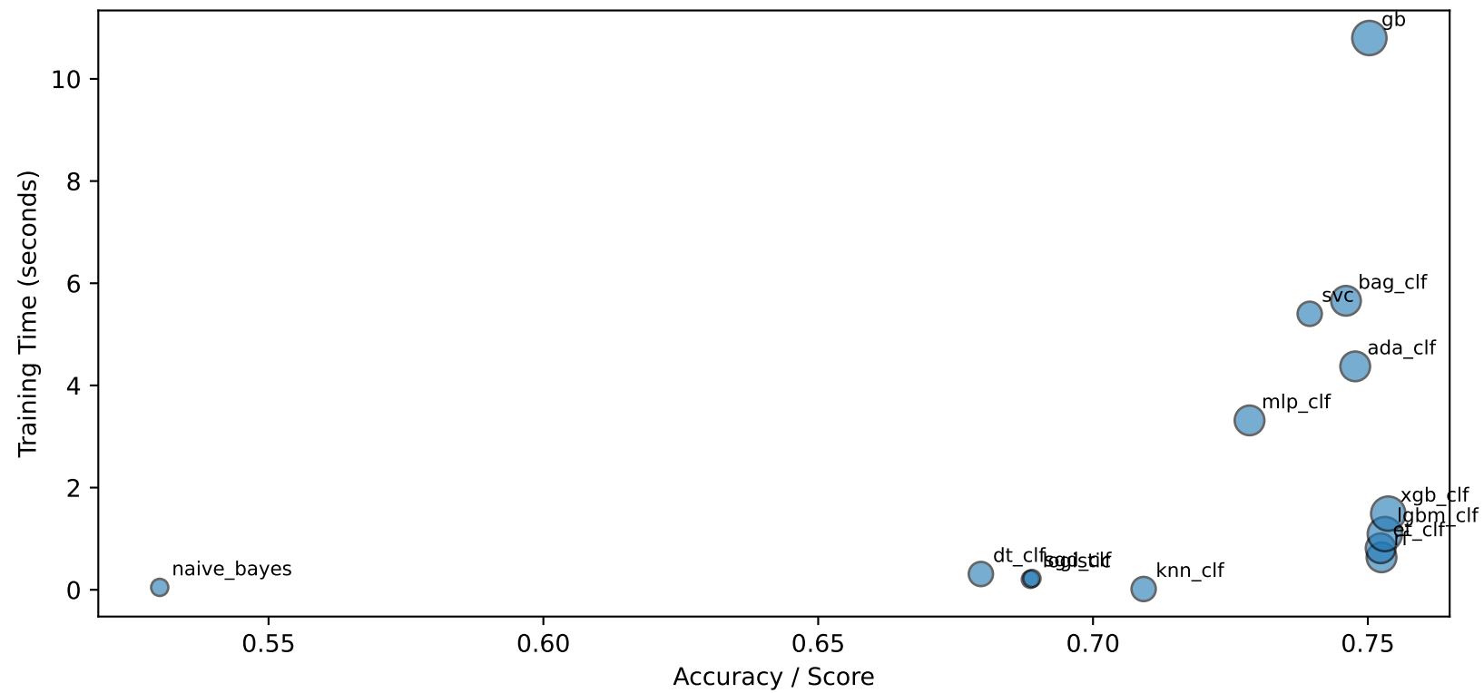
Dataset 4134 (Classification) - Model Trade-offs
