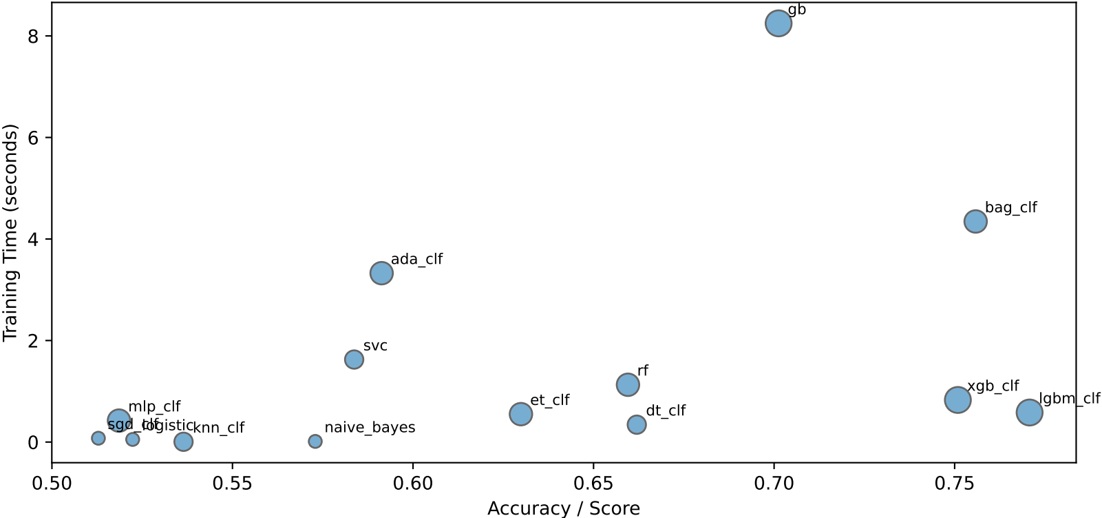
Dataset 1485 (Classification) - Model Trade-offs
