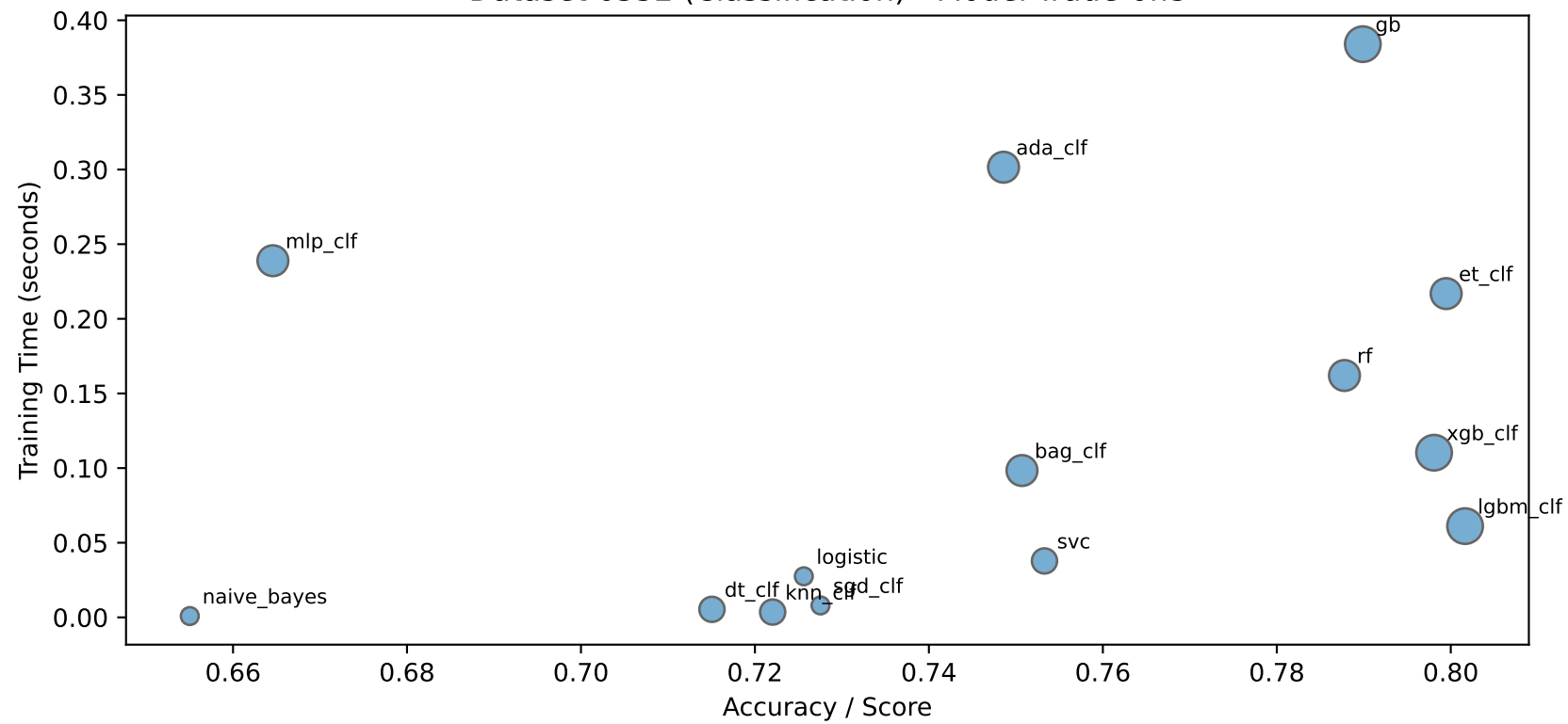
Dataset 6332 (Classification) - Model Trade-offs
