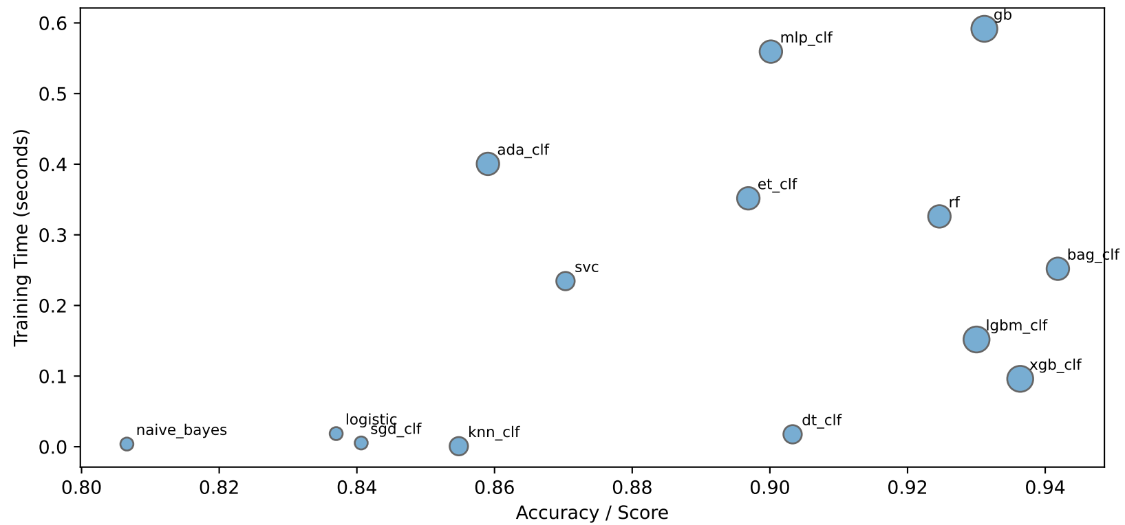
Dataset 40701 (Classification) - Model Trade-offs
