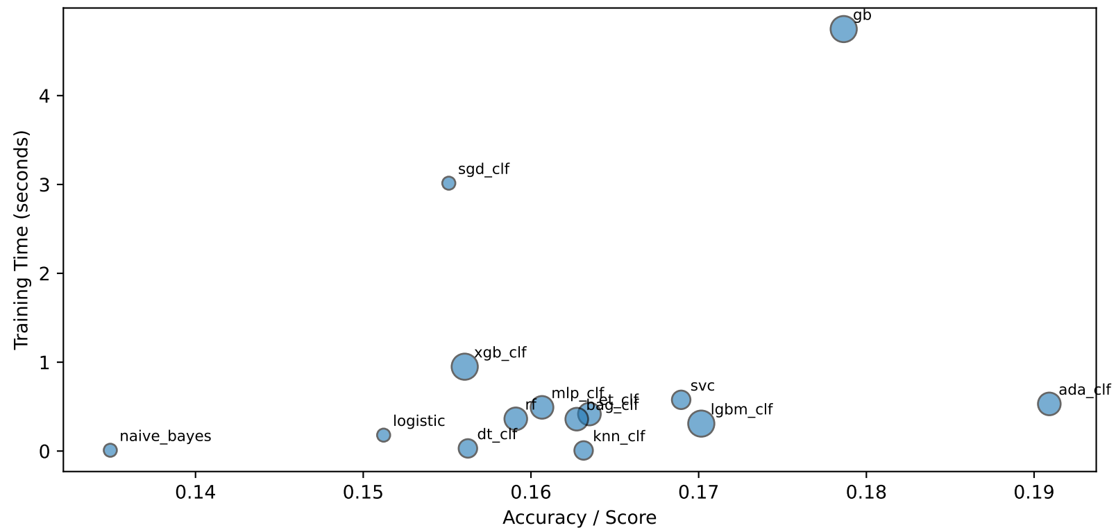
Dataset 1468 (Classification) - Model Trade-offs
