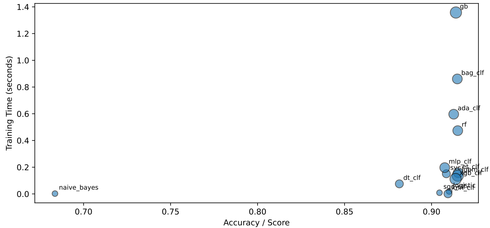
Dataset 1487 (Classification) - Model Trade-offs
