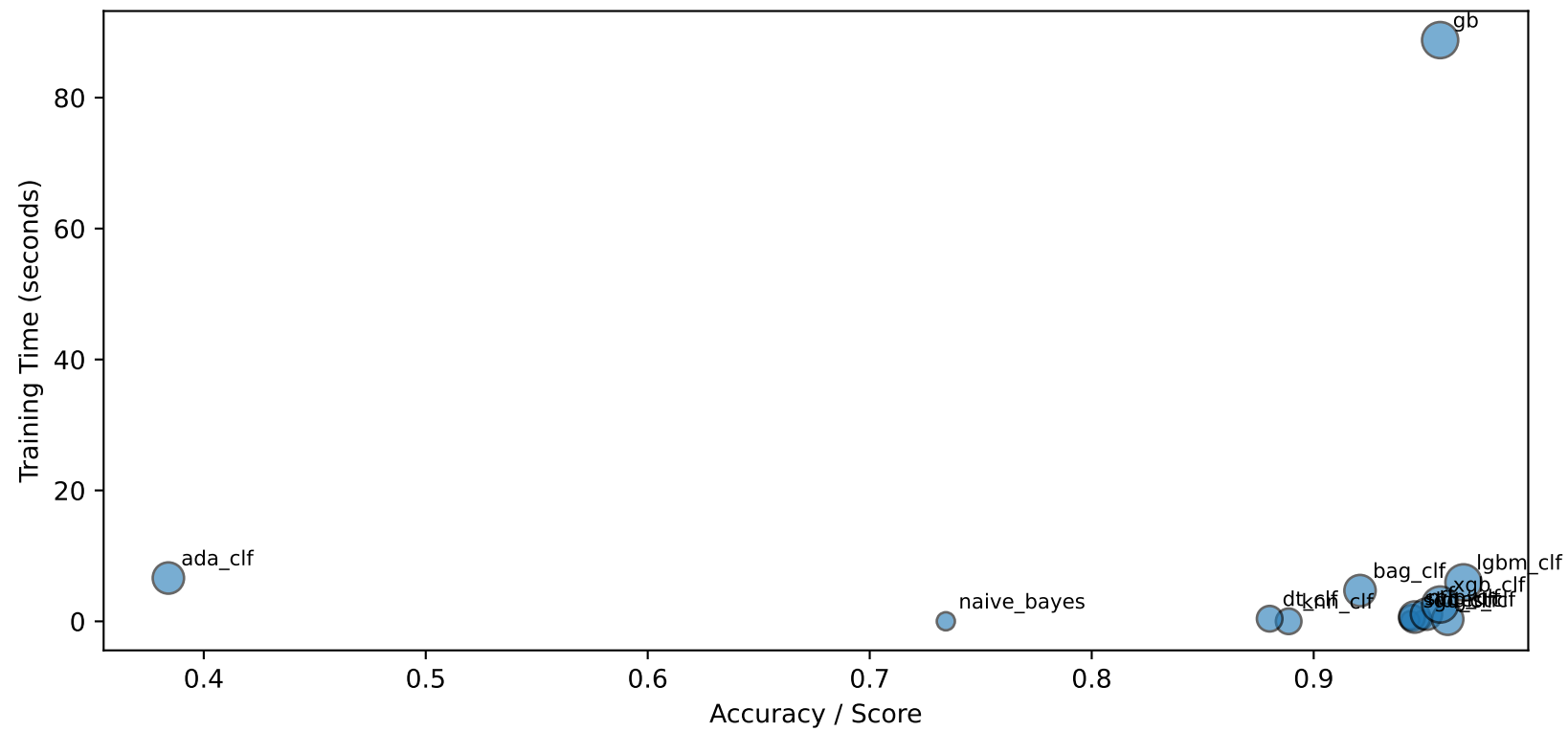
Dataset 1478 (Classification) - Model Trade-offs
