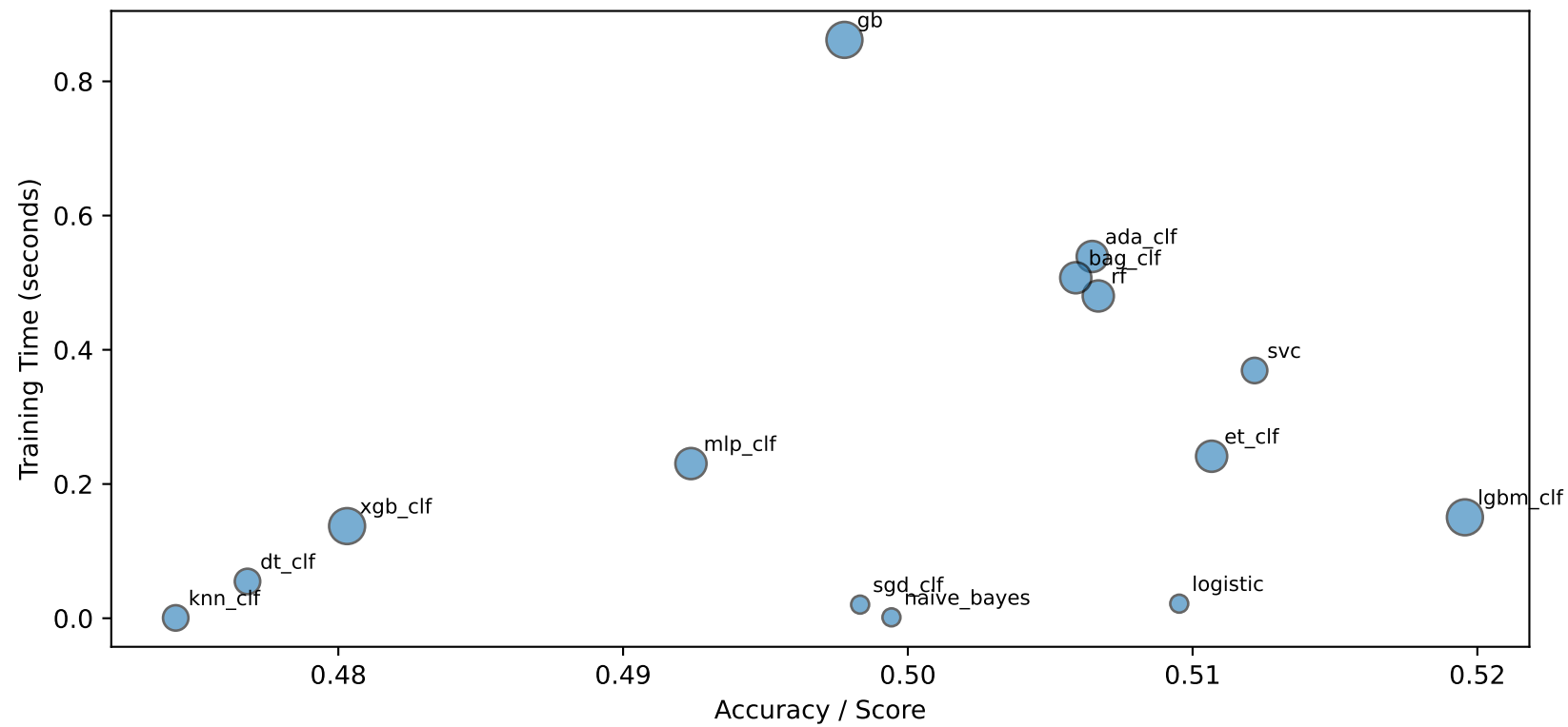
Dataset 23517 (Classification) - Model Trade-offs
