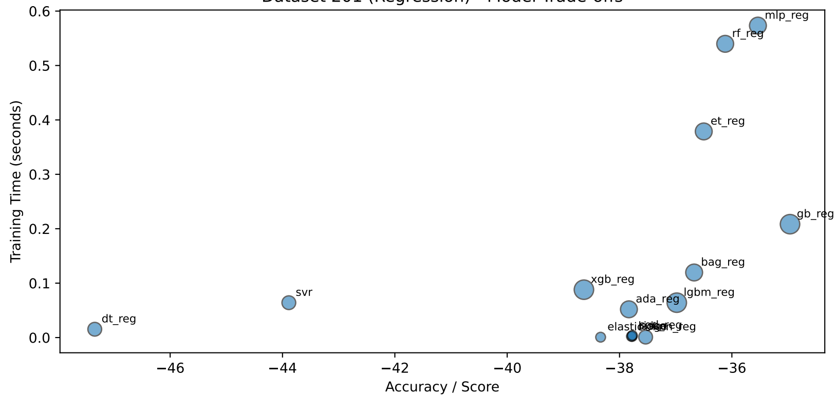
Dataset 201 (Regression) - Model Trade-offs
