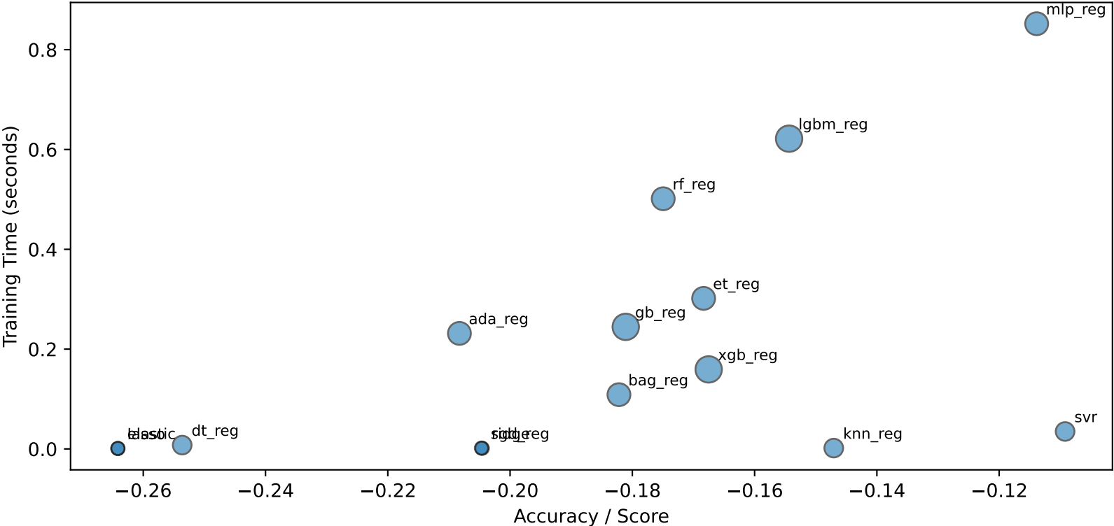
Dataset 189 (Regression) - Model Trade-offs
