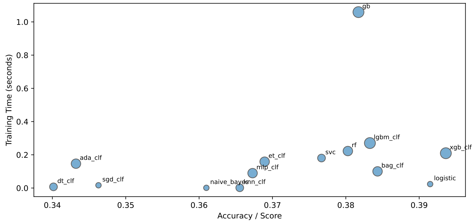
Dataset 40691 (Classification) - Model Trade-offs
