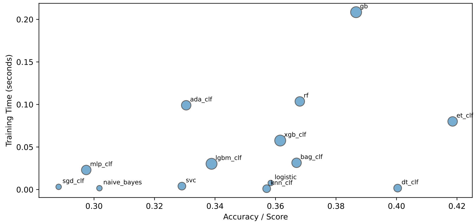
Dataset 1028 (Classification) - Model Trade-offs
