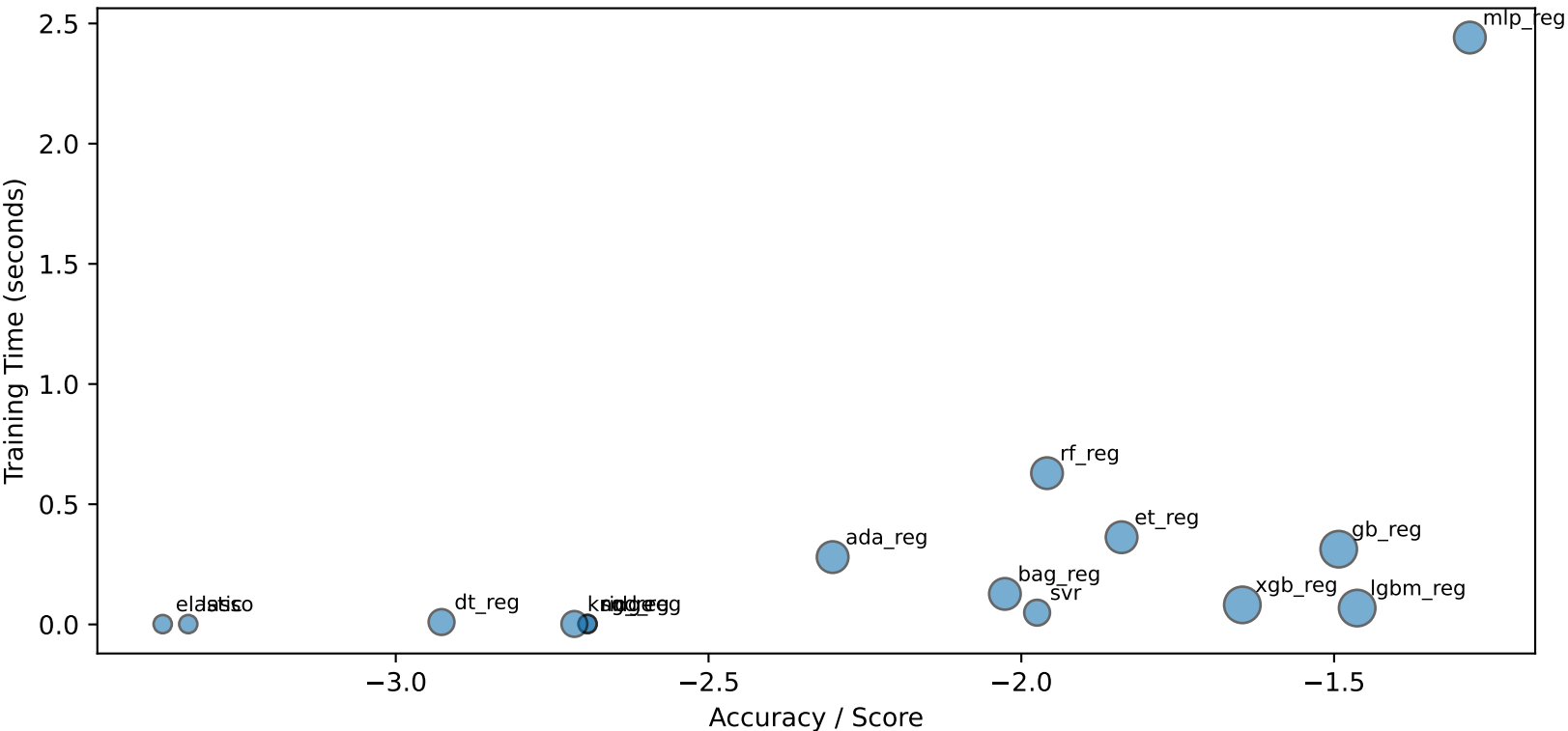
Dataset 564 (Regression) - Model Trade-offs
