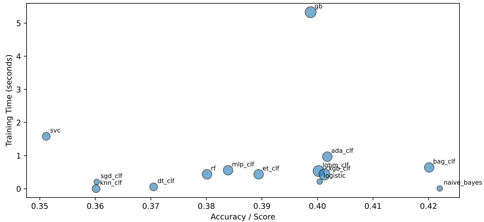
Dataset 40670 (Classification) - Model Trade-offs
