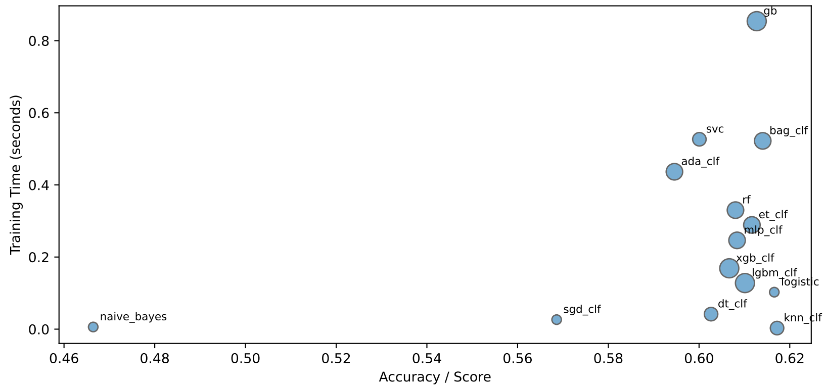
Dataset 1486 (Classification) - Model Trade-offs
