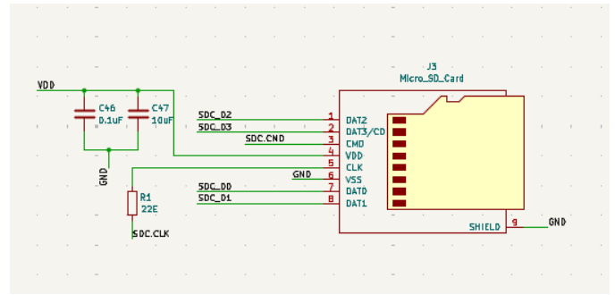
Fig. 6: Micro SD card boot storage schematic.
