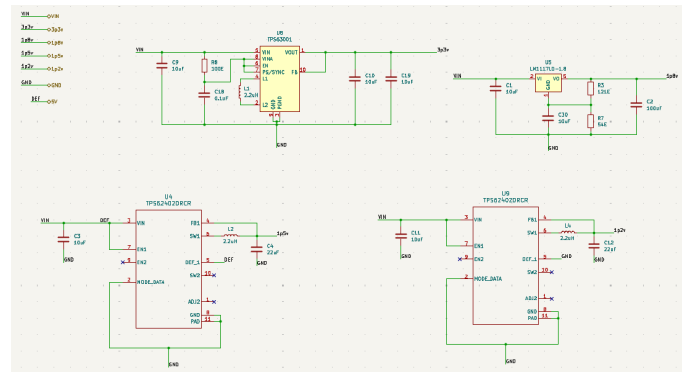
Fig. 7: Power management section generating required voltage rails.
