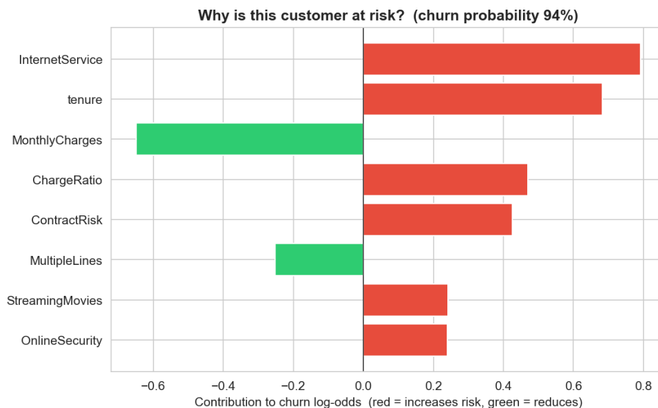
Figure 5 — Per-customer explanation for a high-risk profile (94% churn probability).
