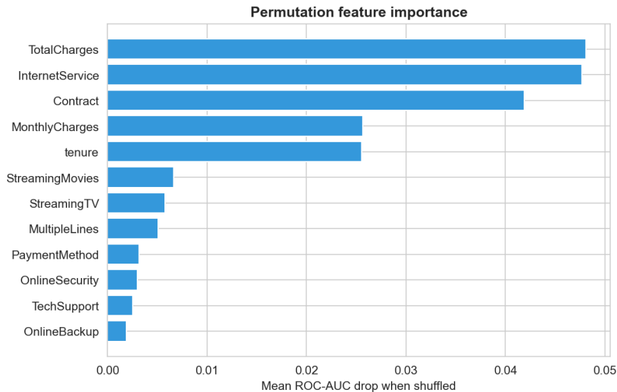
Figure 4 — Permutation feature importance for the deployed model.
