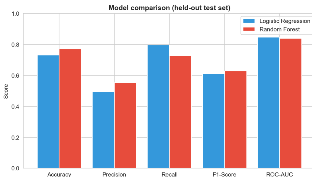
Figure 1 — Model comparison on the held-out test set.
