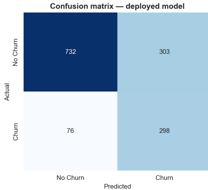
Figure 2 — Confusion matrix of the deployed model; the bottom-right cell is the churners correctly caught.
