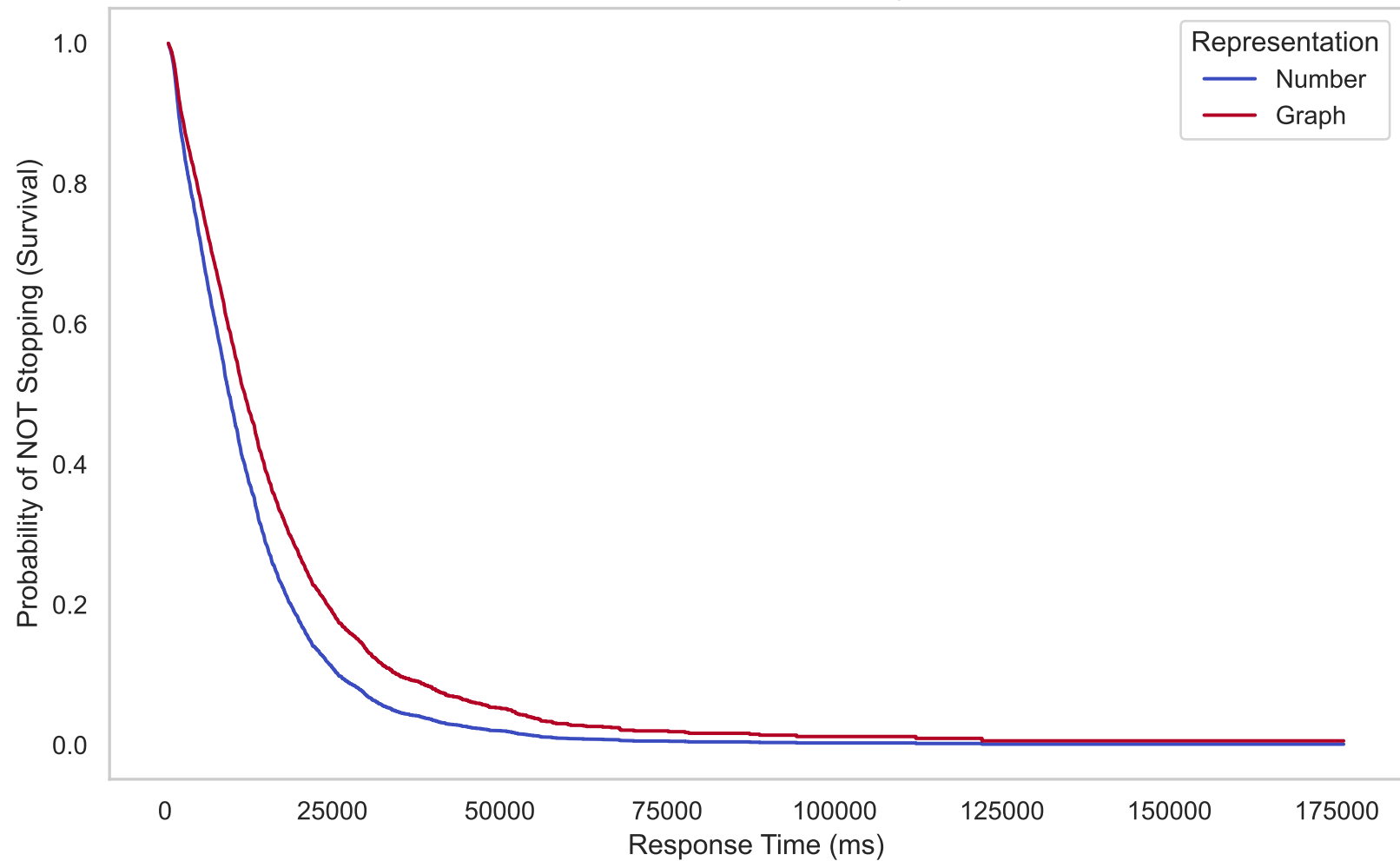
Cox Model Estimated Survival Curves by Representation
