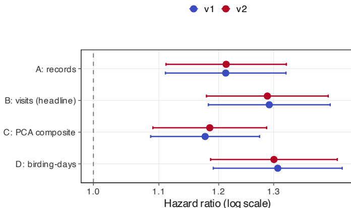
Figure 2 — Province-scale climate × effort interaction is robust to model spec, effort metric, and v1↔v2 refit
