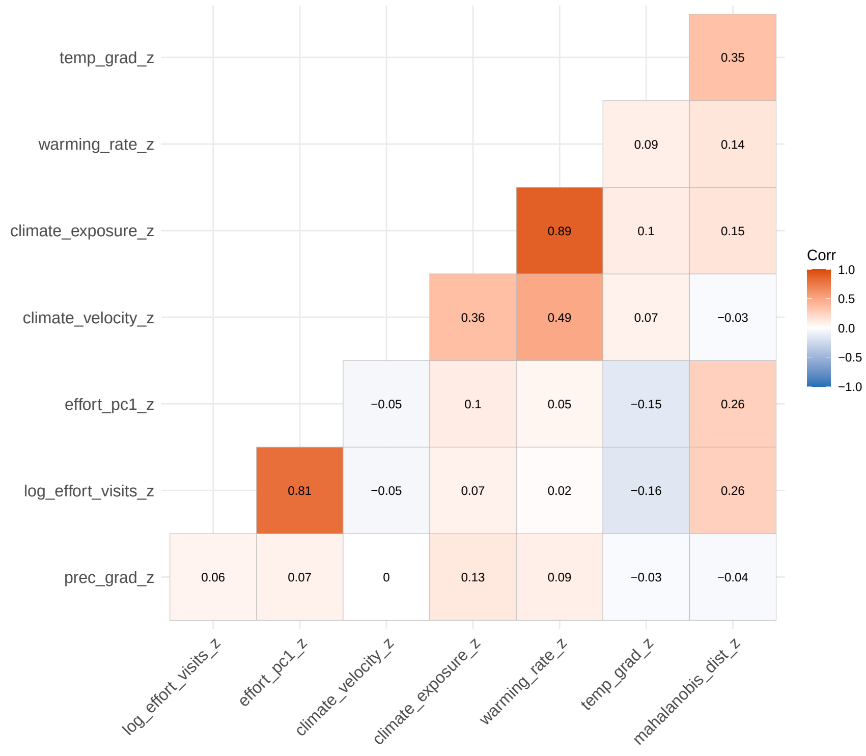
Correlation matrix: climate and effort metrics
