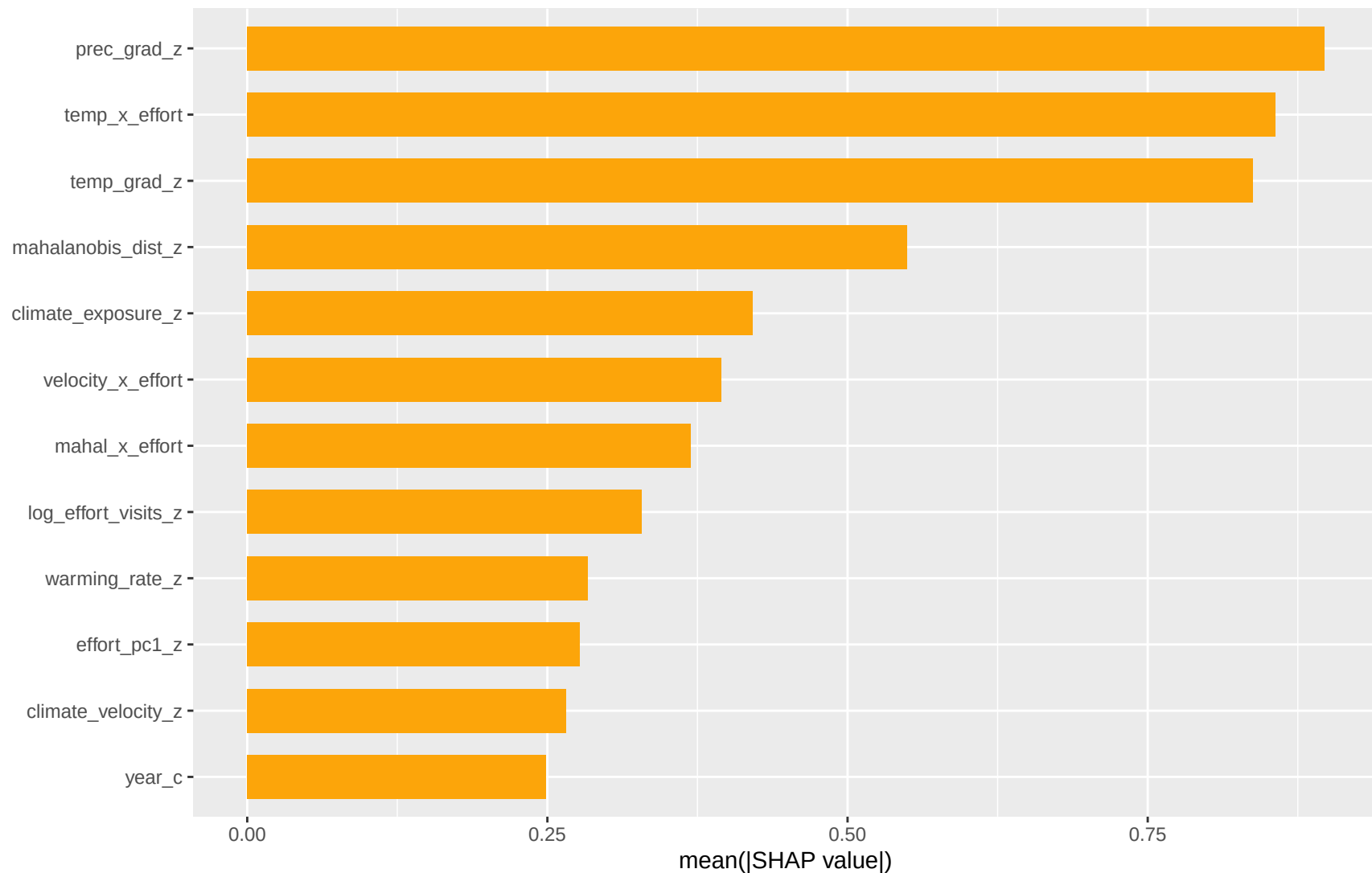
Mean |SHAP| feature importance
