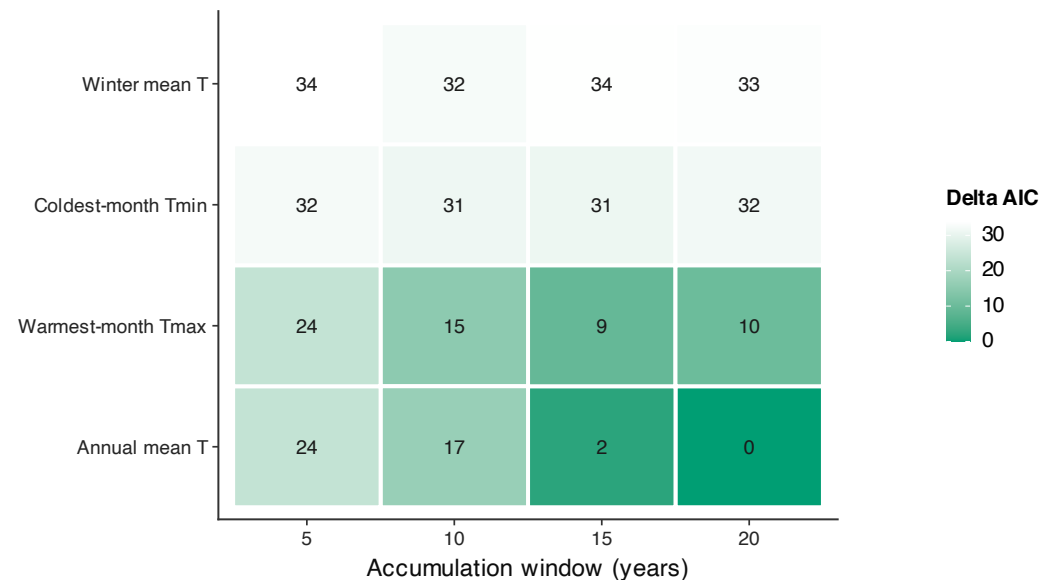
b Model support across climate specifications Delta AIC relative to the best cell; all fitted on the same rows
