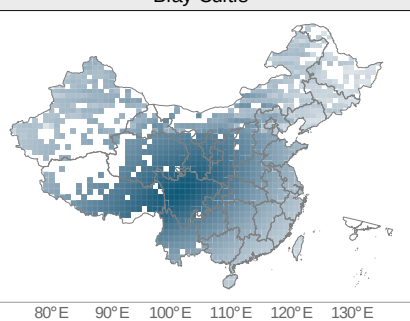
Bray-Curtis
