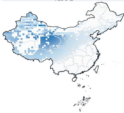
Rao's Q
