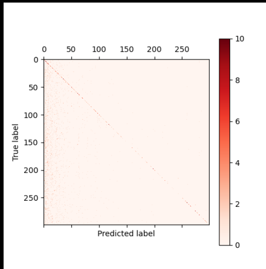
Bonus-300 Acc-15.86%
