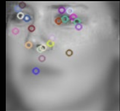
Enhance Brightness
