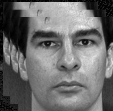
Training samples
