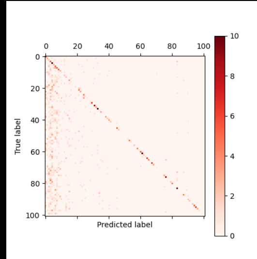
Bonus-100 Acc-24.68%
