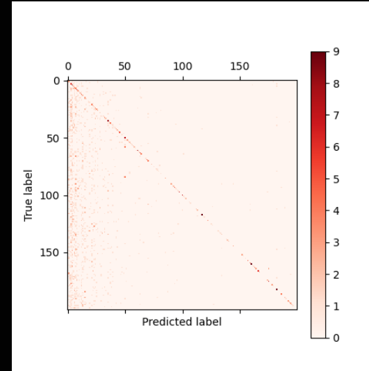
Bonus-200 Acc-18.90%
