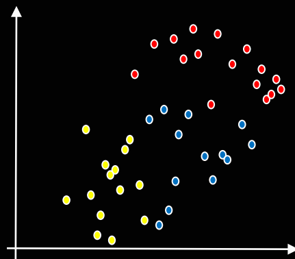
KNN model
