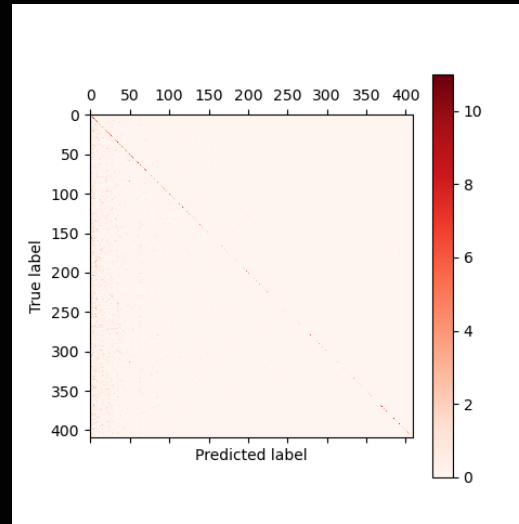
Bonus-400 Acc-14.45%
