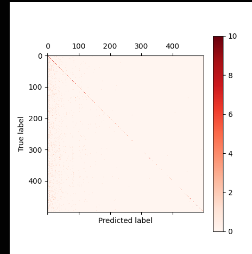
Bonus-500 Acc-14.15%
