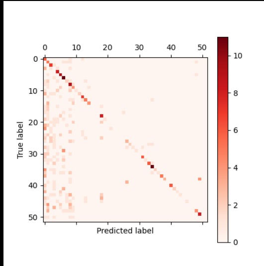
Bonus-50 Acc-33.61%
