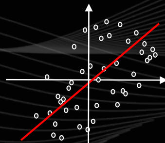
SVM model
