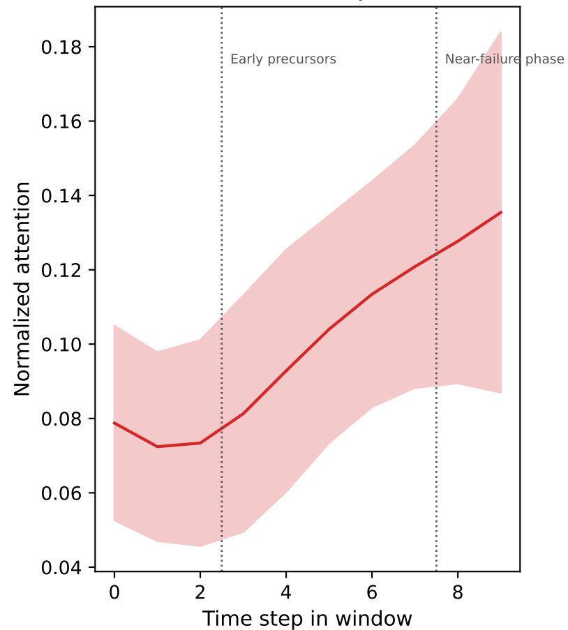
UR3 attention profile
