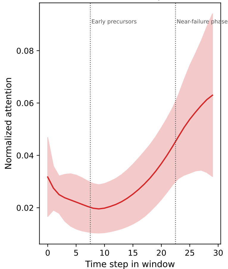
FD001 attention profile
