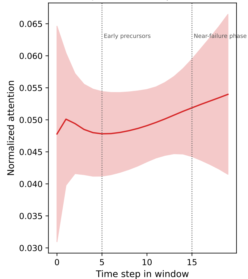
XJTU attention profile
