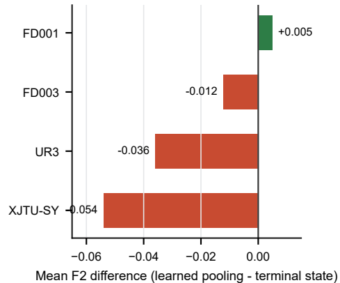
Full-size aggregation contrast
