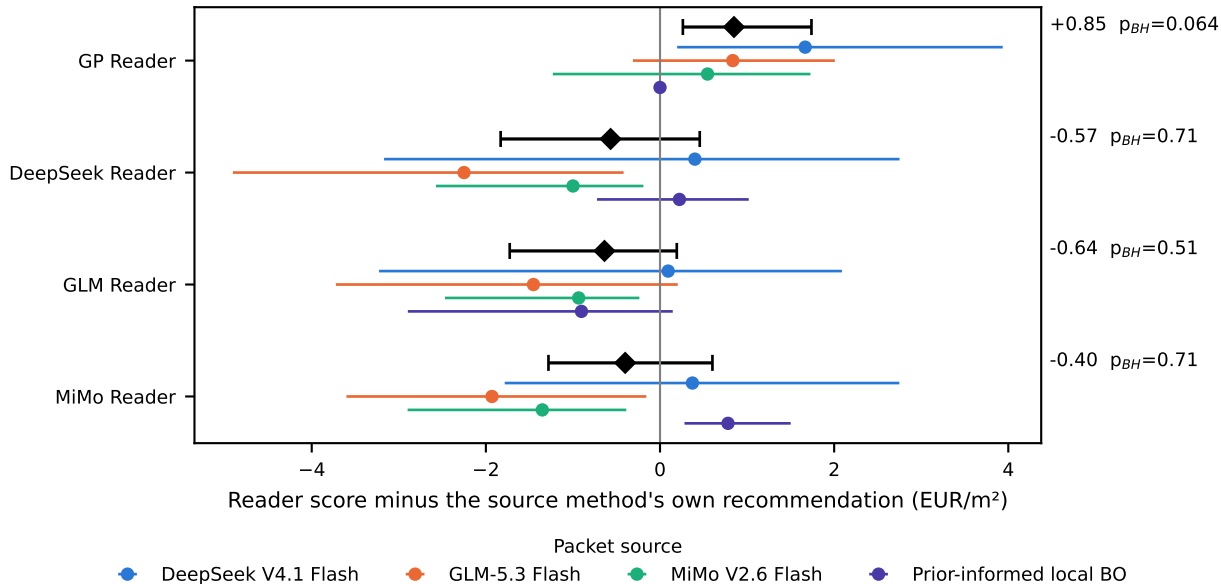
E3: one-shot Readers on the same history packets (diamond: pooled over sites)
