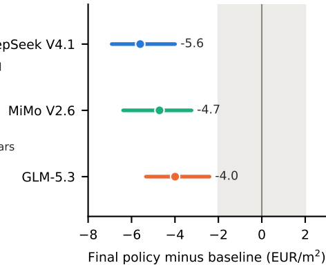
48 sites, all p_{Holm} < 0.001
