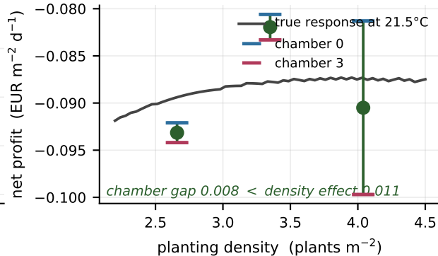
(d) Design B can separate chamber from treatment
