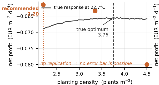
(c) Design A has no way to check itself
