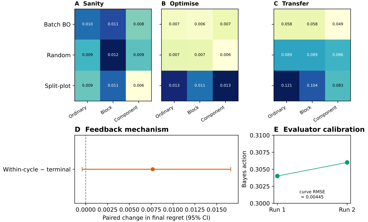
Figure 3: Mechanism checks behind the endpoint comparisons. (A–C) Fixed-history design–reader crossings for SANITY, OPTIMISE and TRANSFER; rows change the executed scripted design and columns change only evidence use. Each cell averages eight held-out sites. Color scales are independent across panels and the annotations give mean realized regret. (D) Registered paired effect of within-cycle access; positive is worse. (E) Two independent factorized evaluator runs select nearly identical Bayes actions; the annotation reports response-curve disagreement.
