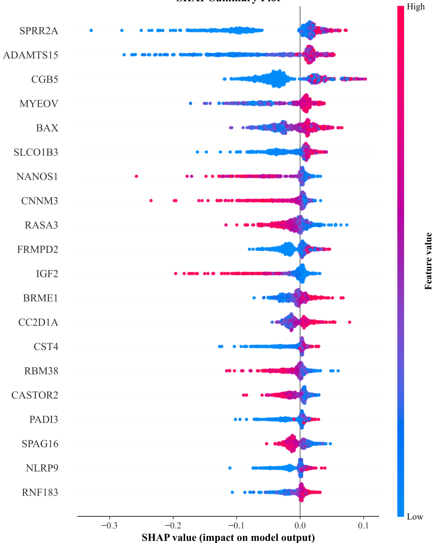
SHAP Summary Plot
