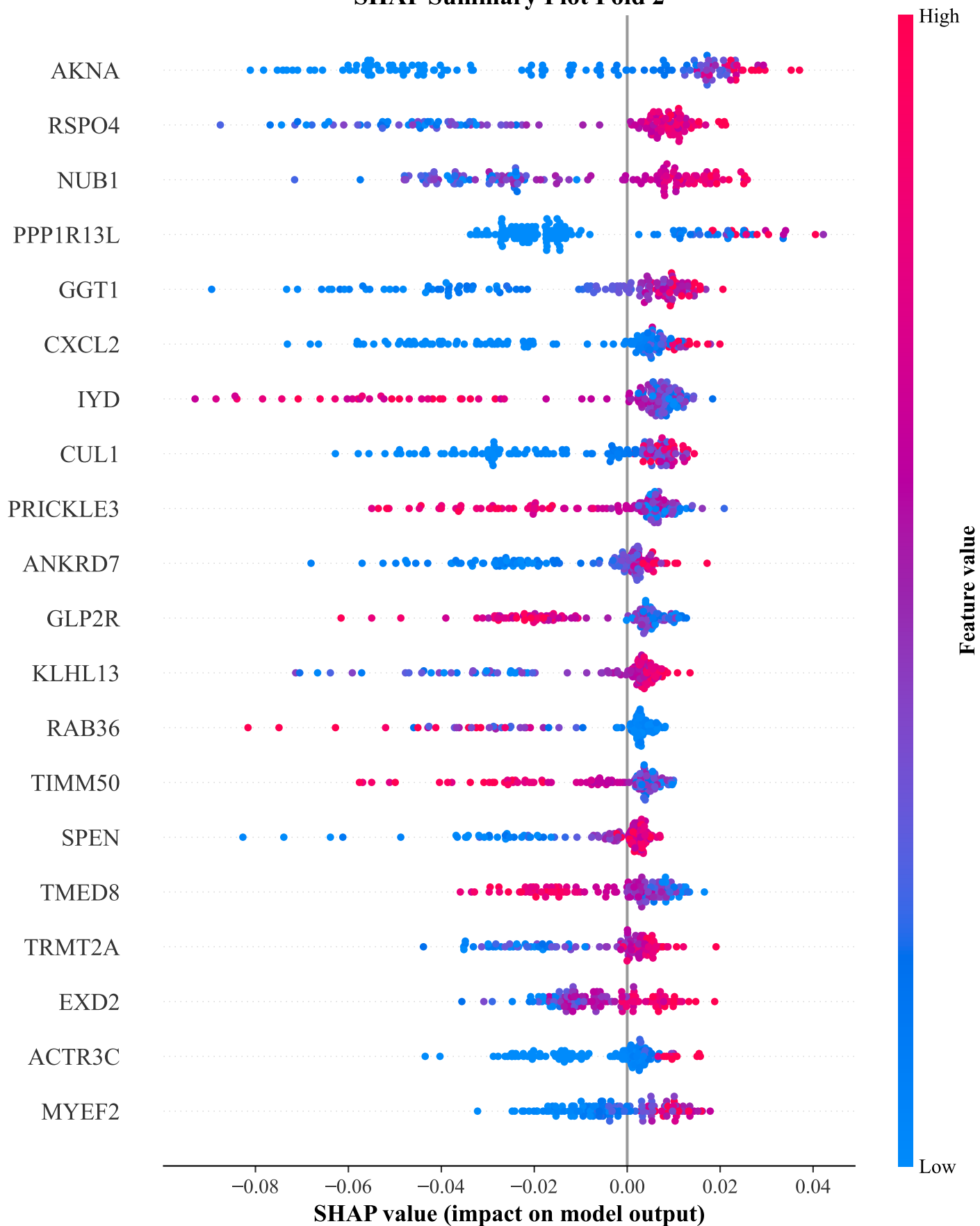
SHAP Summary Plot Fold 2
