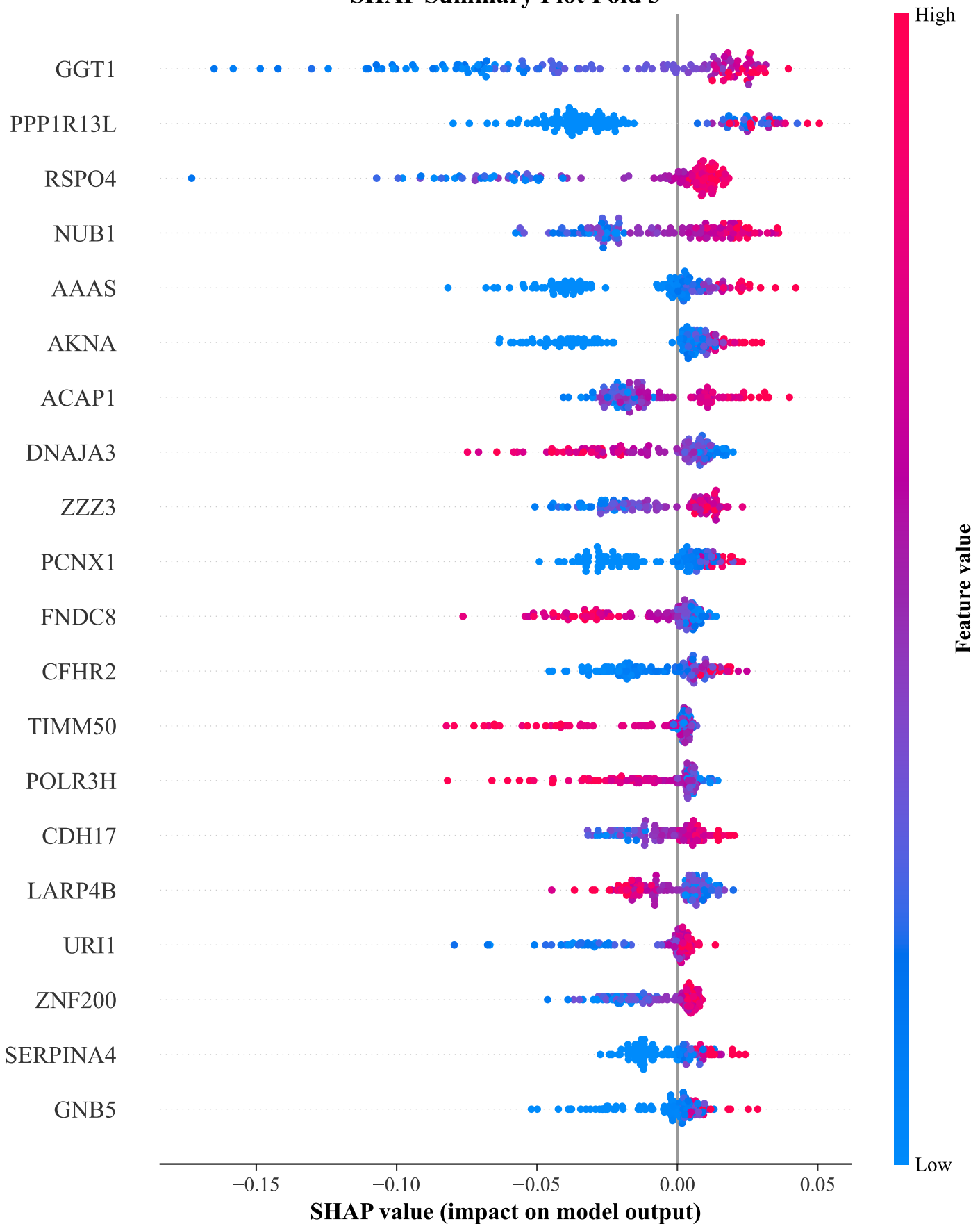
SHAP Summary Plot Fold 3
