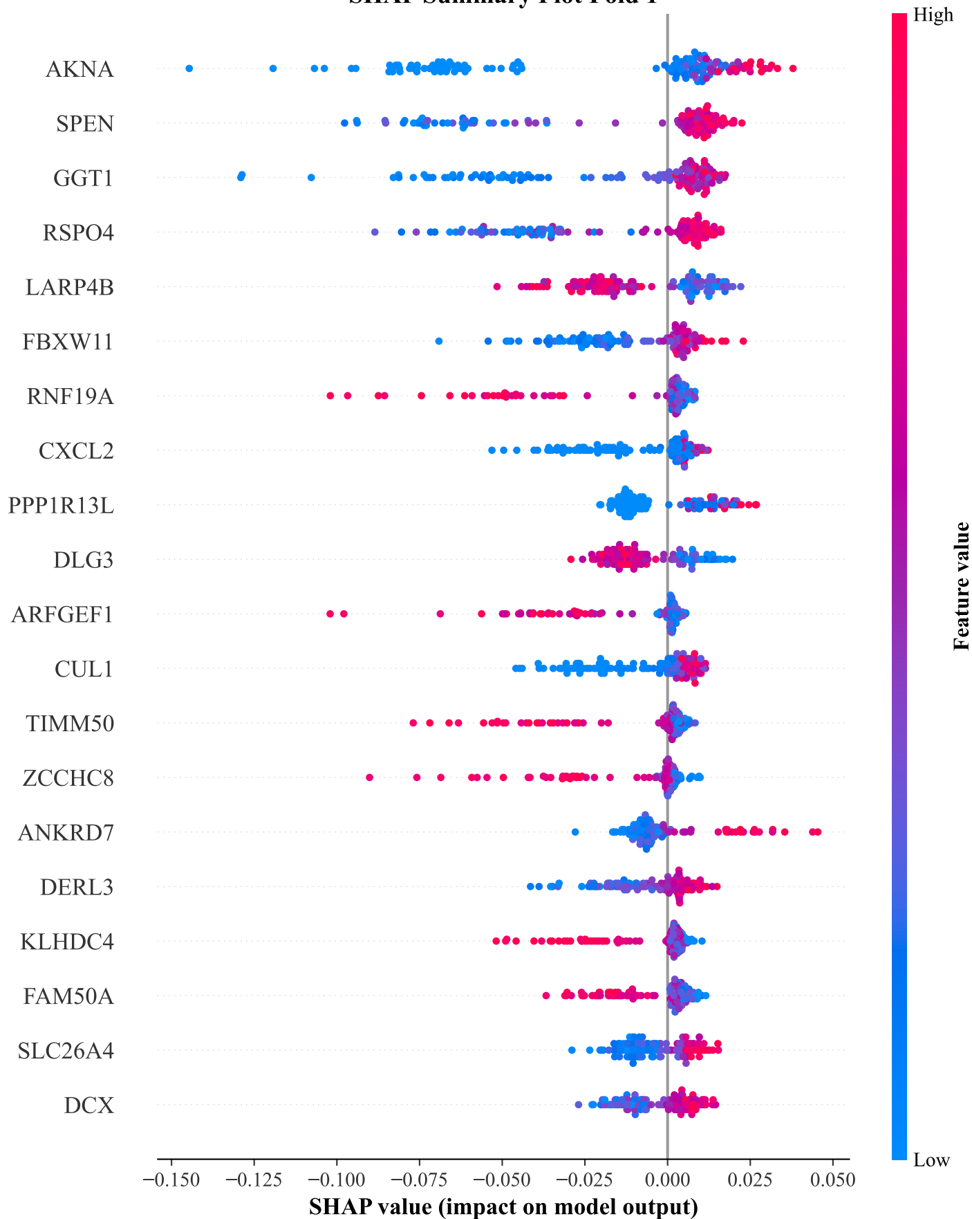
SHAP Summary Plot Fold 1
